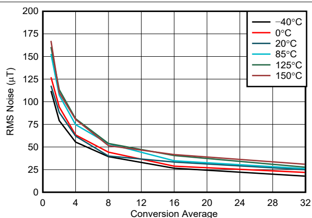
図 5-2. X, Y-Axis Noise vs Conversion Average, 25-mT Range
