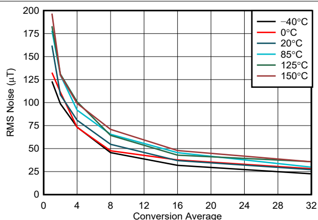
図 5-4. X, Y-Axis Noise vs Conversion Average, 50-mT Range
