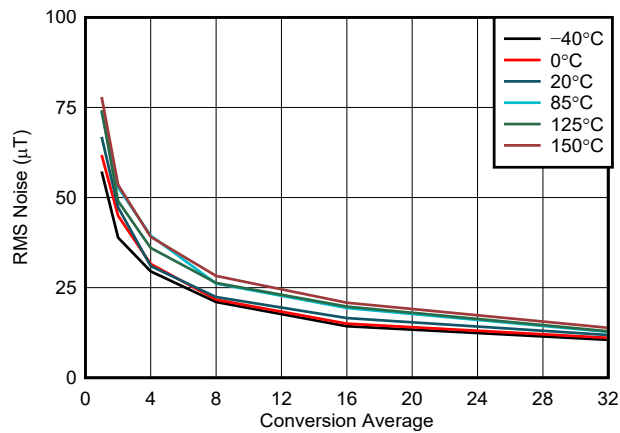
図 5-7. Z-Axis Noise vs Conversion Average, 100-mT Range
