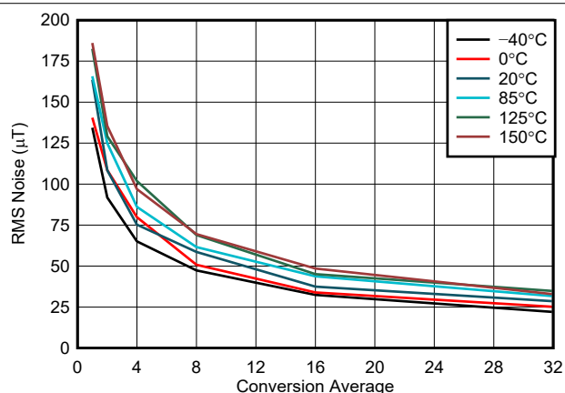
図 5-6. X, Y-Axis Noise vs Conversion Average, 75-mT Range
