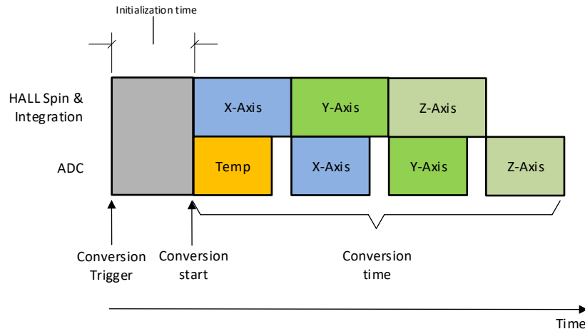
図 7-2. Trigger Conversion for X, Y, Z, and Temperature Sensors
