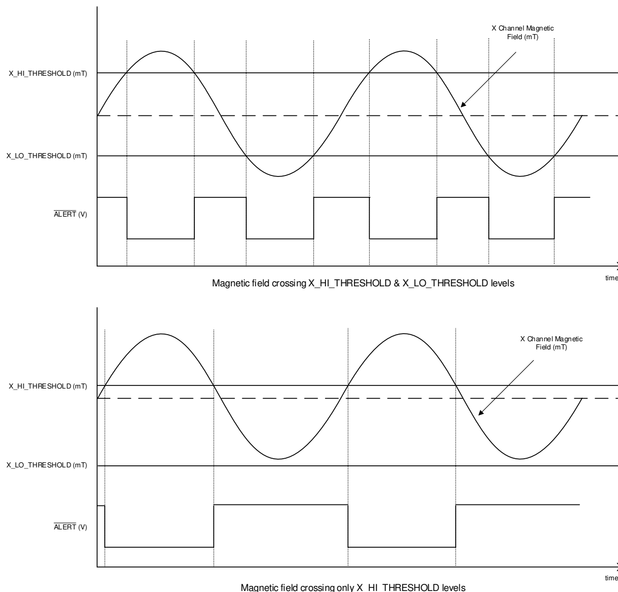
図 6-3. ALERT Pin Working as Magnetic Switch
