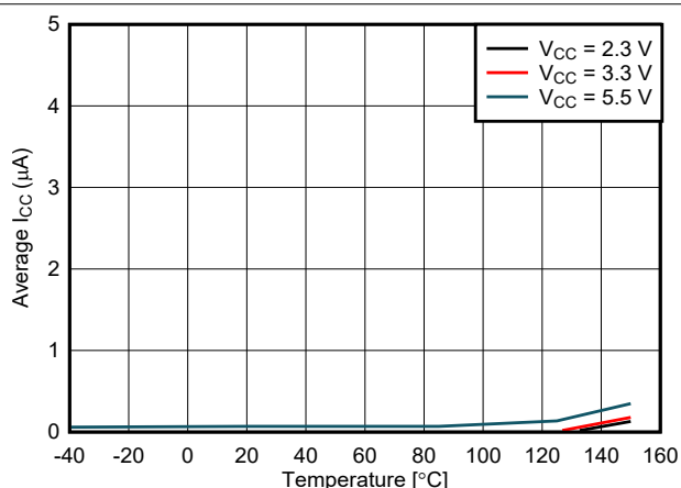
図 5-18. Deep Sleep Mode Supply Current vs Temperature
