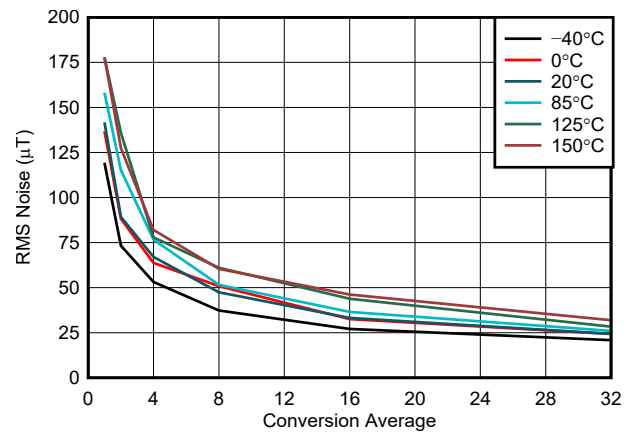
図 5-8. X, Y-Axis Noise vs Conversion Average, 100-mT Range
