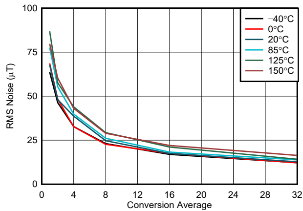
図 5-9. Z-Axis Noise vs Conversion Average, 150-mT Range
