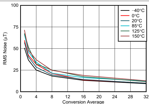
図 5-1. Z-Axis Noise vs Conversion Average, 25-mT Range
