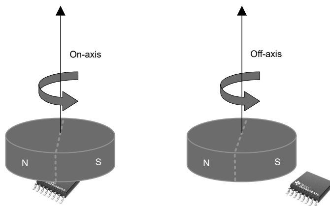
図 7-5. On-Axis vs. Off-Axis Angle Measurements
