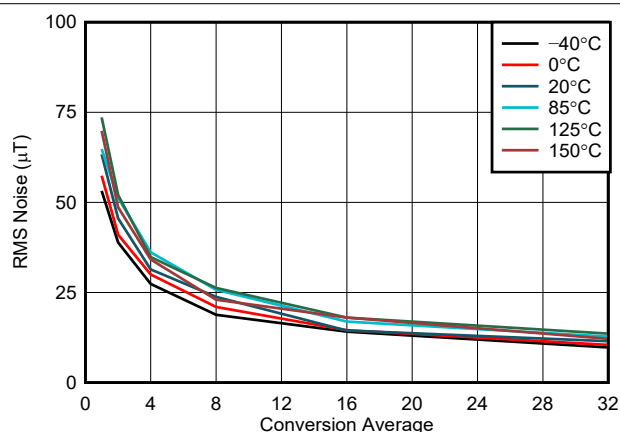
図 5-5. Z-Axis Input vs Conversion Average, 75-mT Range
