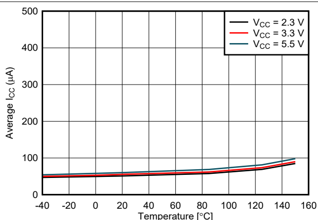
図 5-16. Configuration Mode Supply Current vs Temperature
