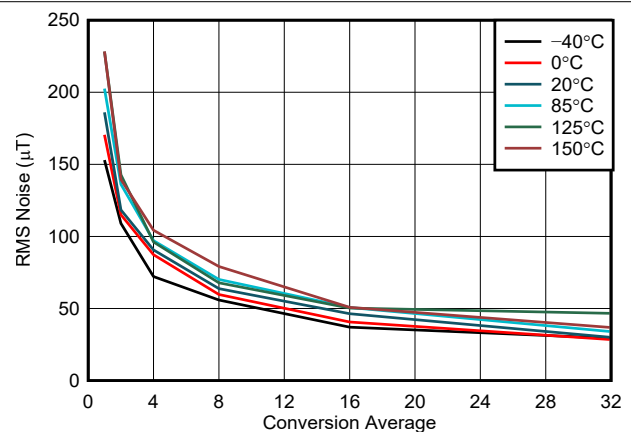
図 5-12. X, Y-Axis Noise vs Conversion Average, 300-mT Range
