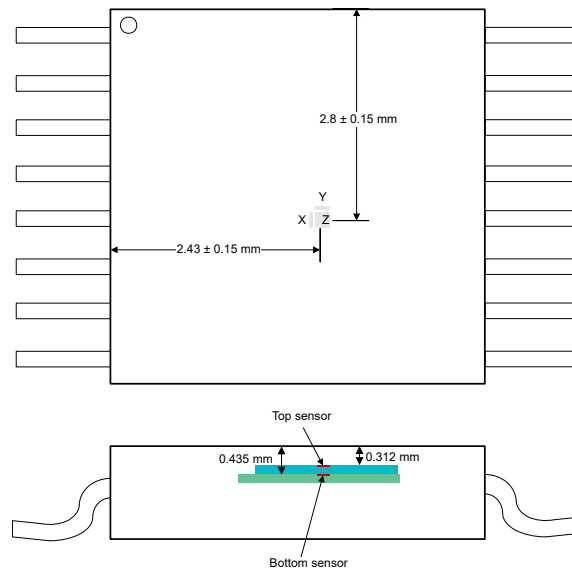
図 6-2. Location of X, Y, Z Hall Elements
