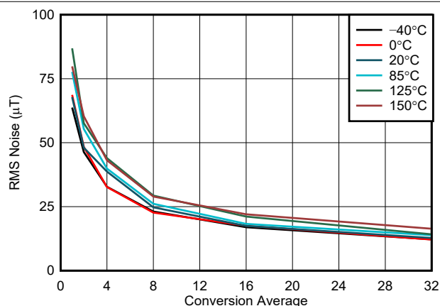
図 5-3. Z-Axis Noise vs Conversion Average, 50-mT Range
