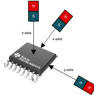
図 6-1. Direction of Applied Magnetic South Pole to Generate Positive ADC Codes
