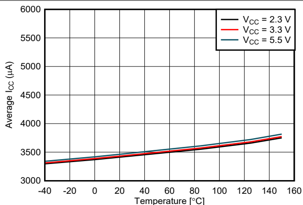
図 5-14. Active Mode Supply Current vs Temperature
