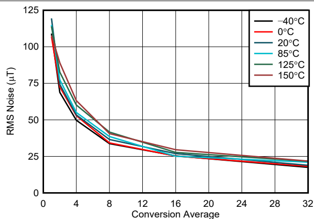
図 5-11. Z-Axis Noise vs Conversion Average, 300-mT Range
