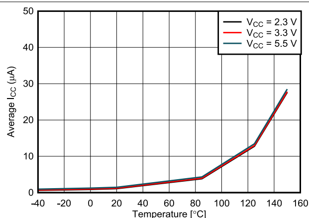
図 5-17. Sleep Mode Supply Current vs Temperature
