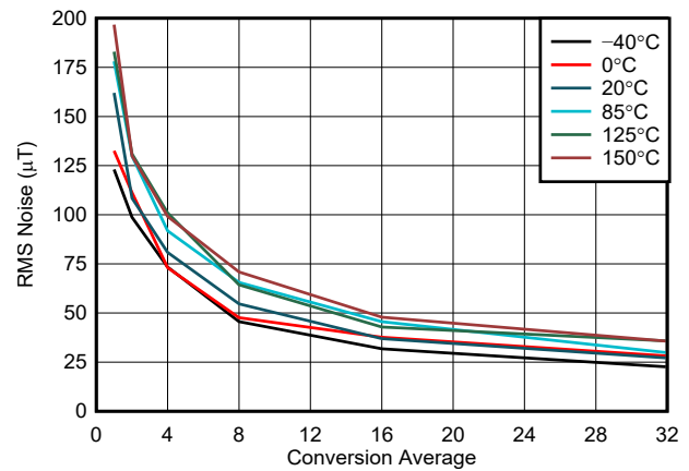
図 5-10. X, Y-Axis Noise vs Conversion Average, 150-mT Range
