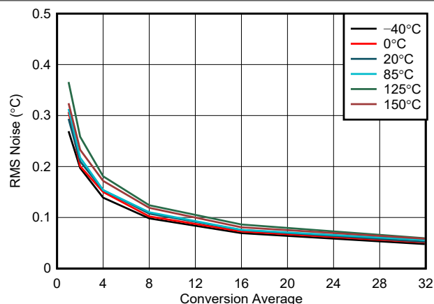
図 5-13. Temperature Sensor Noise vs Conversion Average
