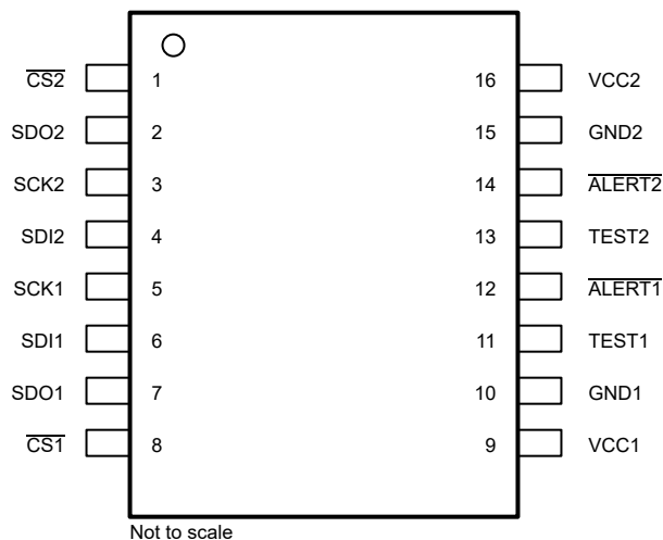
図 4-1. PW Package 16-Pin TSSOP Top View
