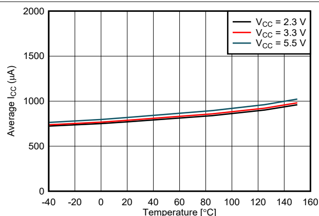
図 5-15. Standby Mode Supply Current vs Temperature
