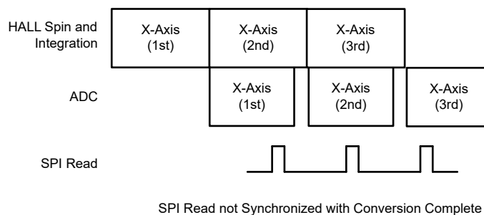
7-8. SPI Read During Continuous Conversion
