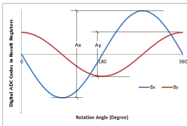
✎ 8-7. X and Y Sensor Data for Full 360 Degree Rotation for Off-Axis Measurement
