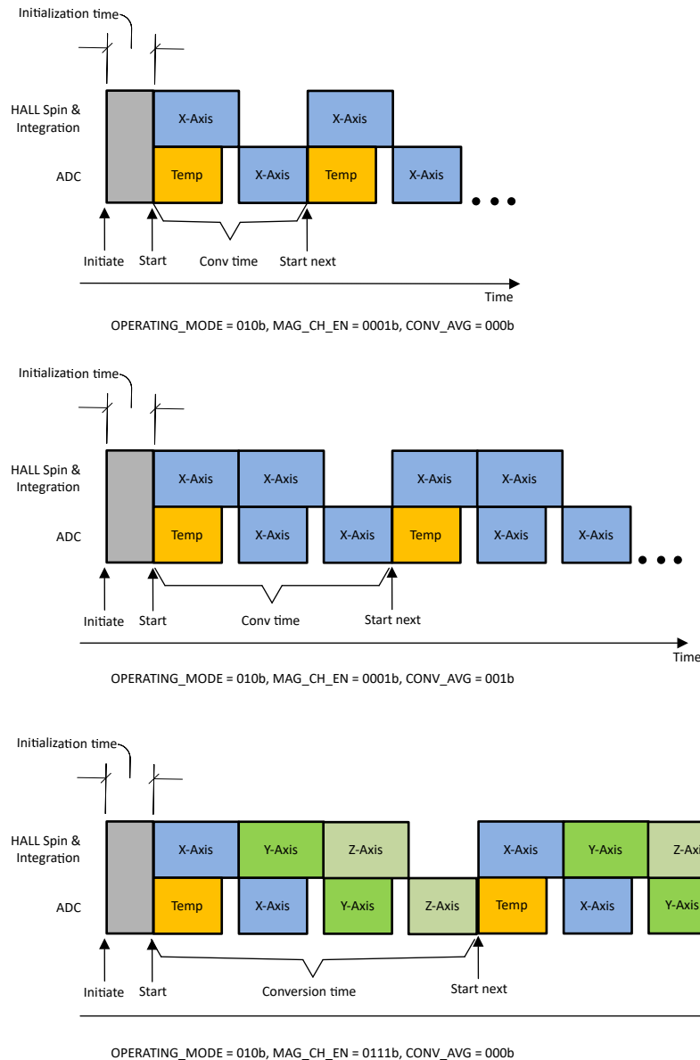
8-1. Continuous Conversion Examples
