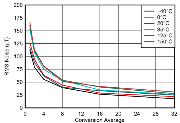
FIG 6-2. X, Y-Axis Noise vs. Conversion Average, 25-mT Range
