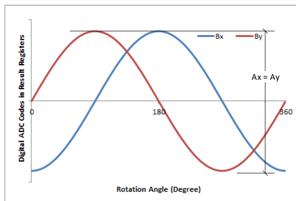
✎ 8-6. X and Y Sensor Data for Full 360 Degree Rotation for On-Axis Measurement
