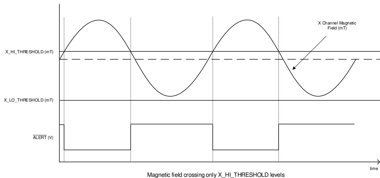
图 7-3. ALERT Pin Working as Magnetic Switch
