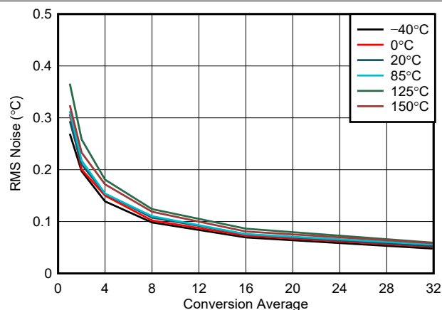
FIG 6-13. Temperature Sensor Noise vs. Conversion Average
