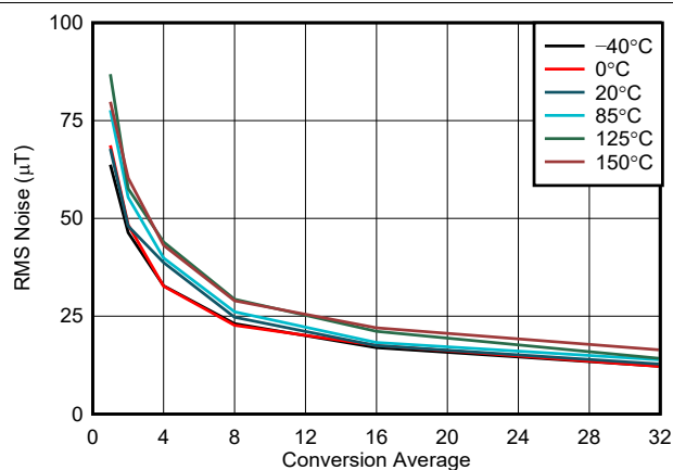
FIG 6-3. Z-Axis Noise vs. Conversion Average, 50-mT Range
