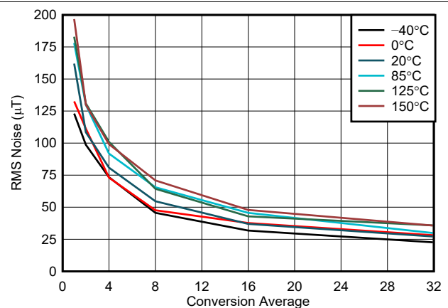
FIG 6-4. X, Y-Axis Noise vs. Conversion Average, 50-mT Range
