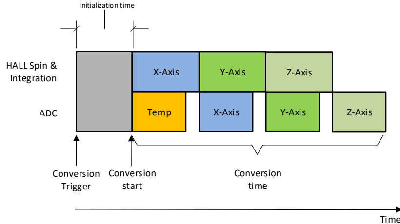
8-2. Trigger Conversion for X, Y, Z, and Temperature Sensors
