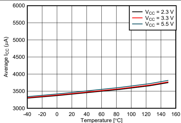
FIG 6-14. Active Mode Supply Current vs. Temperature
