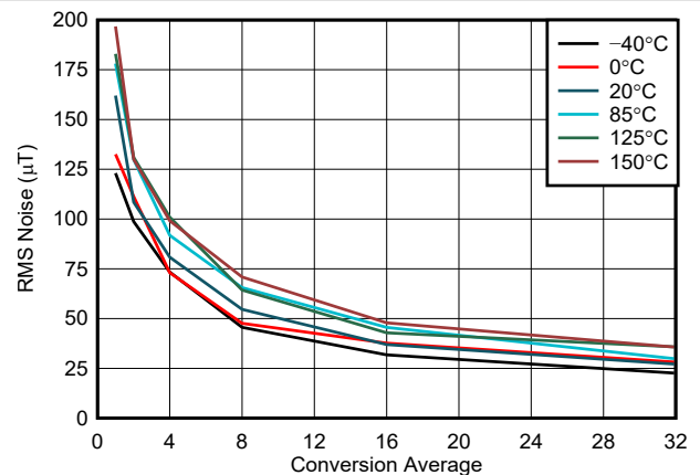
FIG 6-10. X, Y-Axis Noise vs. Conversion Average, 150-mT Range
