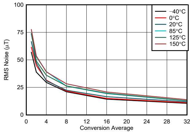
FIG 6-7. Z-Axis Noise vs. Conversion Average, 100-mT Range
