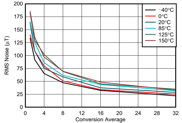
FIG 6-6. X, Y-Axis Noise vs. Conversion Average, 75-mT Range
