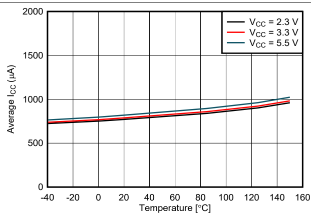
FIG 6-15. Standby Mode Supply Current vs. Temperature
