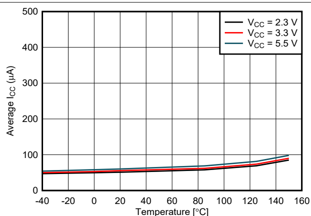
FIG 6-16. Configuration Mode Supply Current vs. Temperature
