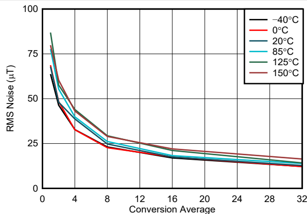
FIG 6-9. Z-Axis Noise vs. Conversion Average, 150-mT Range
