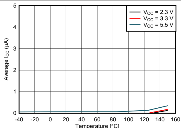
FIG 6-18. Deep Sleep Mode Supply Current vs. Temperature
