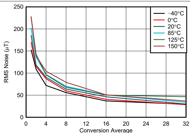
FIG 6-12. X, Y-Axis Noise vs. Conversion Average, 300-mT Range
