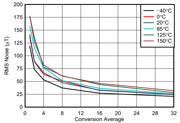
FIG 6-8. X, Y-Axis Noise vs. Conversion Average, 100-mT Range
