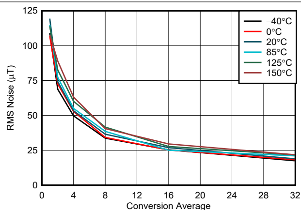
FIG 6-11. Z-Axis Noise vs. Conversion Average, 300-mT Range
