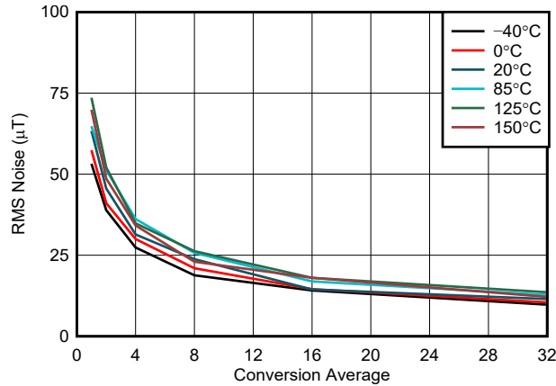
FIG 6-5. Z-Axis Input vs. Conversion Average, 75-mT Range
