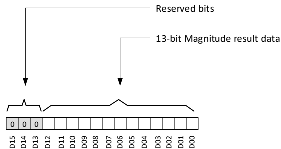
✎ 7-9. Magnitude Result Data Definition
