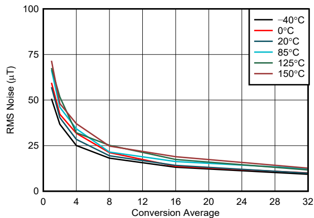
FIG 6-1. Z-Axis Noise vs. Conversion Average, 25-mT Range
