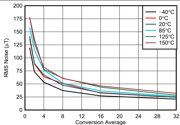
FIG 6-8. X, Y-Axis Noise vs. Conversion Average, 100-mT Range
