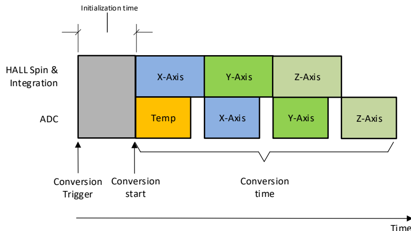
图 8-2. Trigger Conversion for X, Y, Z, and Temperature Sensors
