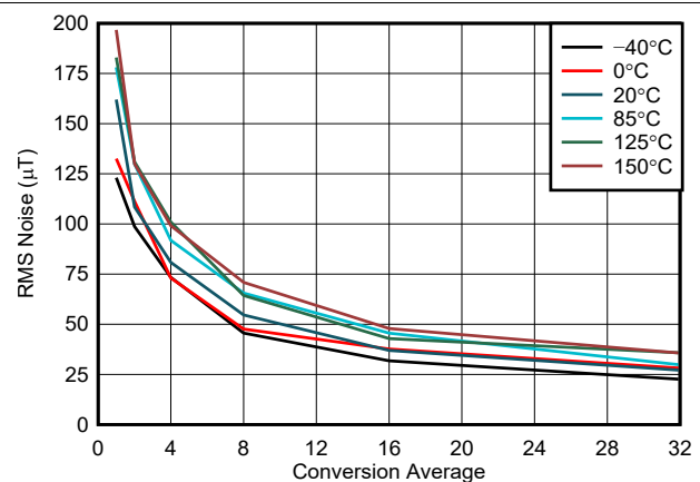
FIG 6-4. X, Y-Axis Noise vs. Conversion Average, 50-mT Range
