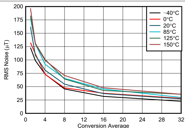
FIG 6-10. X, Y-Axis Noise vs. Conversion Average, 150-mT Range
