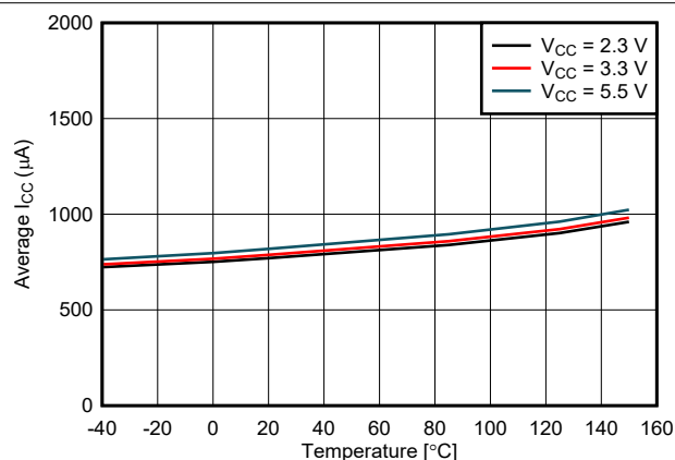
FIG 6-15. Standby Mode Supply Current vs. Temperature
