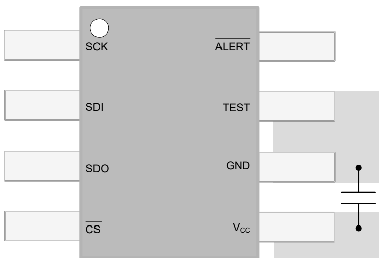
10-1. Layout Example With TMAG5170
