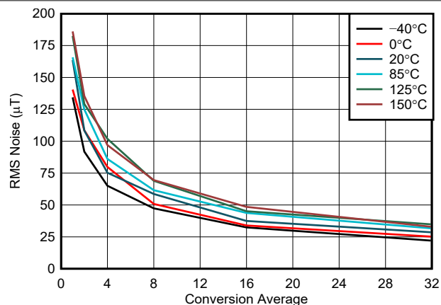
FIG 6-6. X, Y-Axis Noise vs. Conversion Average, 75-mT Range
