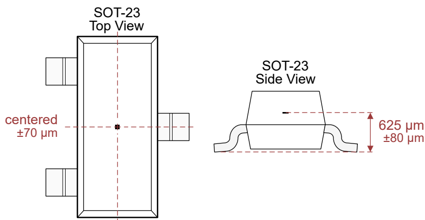
✎ 7-10. Hall Element Location
