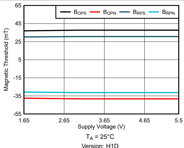
6-10. 37mT B_{Op} : Thresholds vs Supply Voltage
