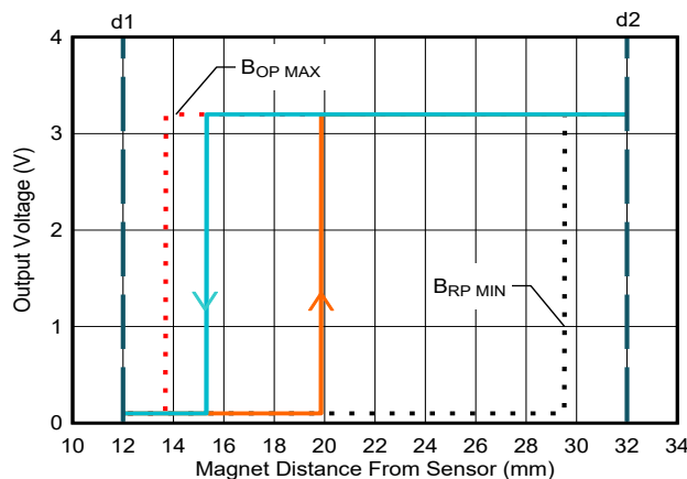
図 8-10. Thresholds From Hypothesis Two
