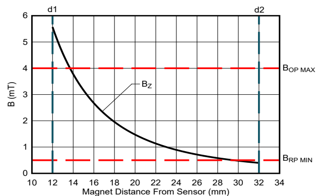
図 8-9. B-Field Hypothesis Two
