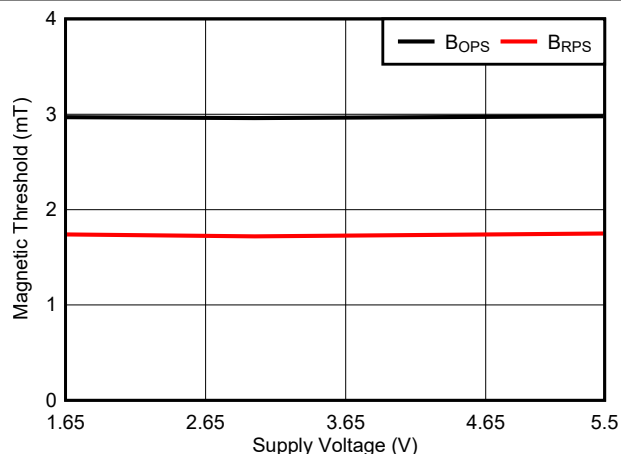
6-6. 3mT B_{OP} , 1.2mT B_{HYS} : Thresholds vs Supply Voltage
