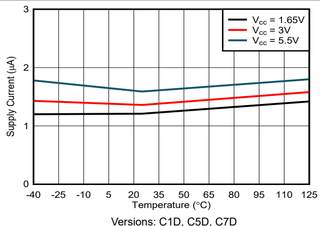
6-12. 20Hz: Average I_{CC} vs Temperature
