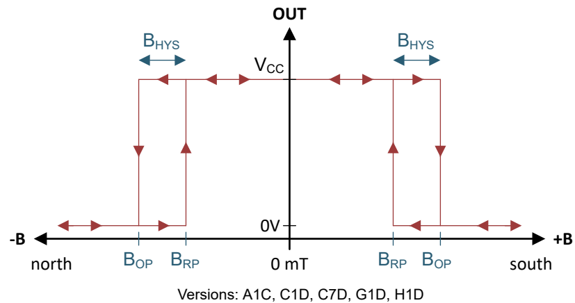
7-5. Omnipolar Active Low Functionality
