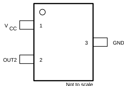
図 5-1. DBZ Package 3-Pin SOT-23 (Top View): A1C, 図 5-2. DBZ Package 3-Pin SOT-23 (Top View): C5D C1D, C7D, G1D, H1D Versions
