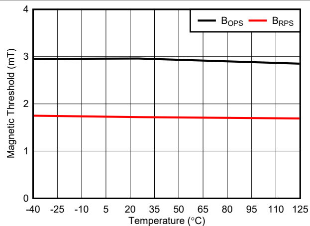
6-5. 3mT B_{OP} , 1.2mT B_{HYS} : Thresholds vs Temperature
