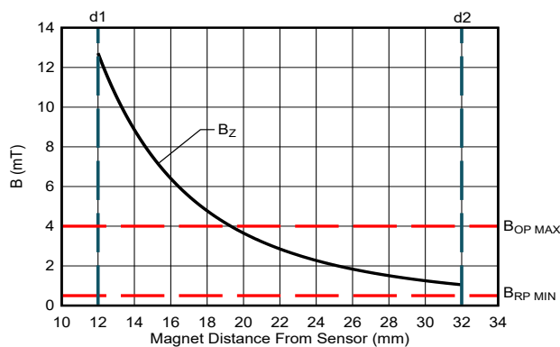
図 8-8. B-Field Hypothesis One
