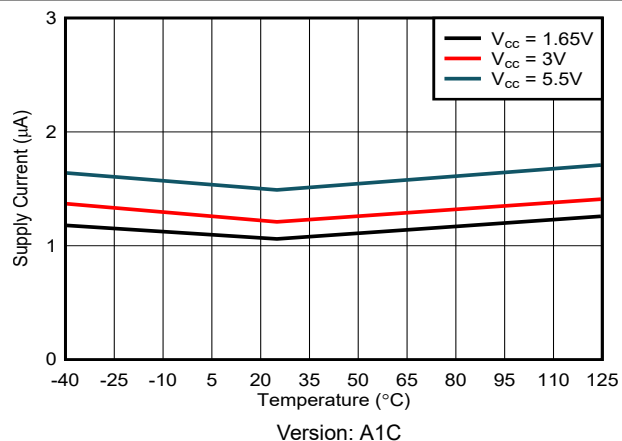
6-11. 10Hz: Average I_{CC} vs Temperature
