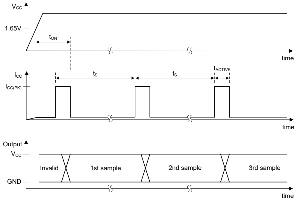
✎ 7-9. Timing Diagram
