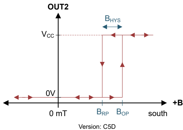
7-6. Unipolar Active High Functionality
