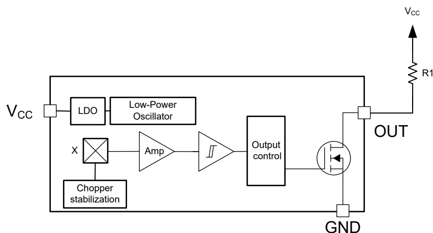
図 7-2. Block Diagram (Open-Drain)
