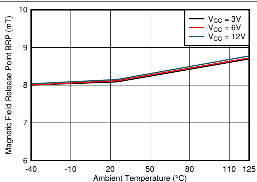
7-15. B_{RP} vs Temperature
