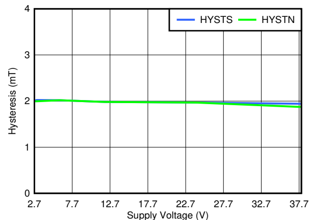
7-6. TMAG5123B Hysteresis vs. Supply Voltage
