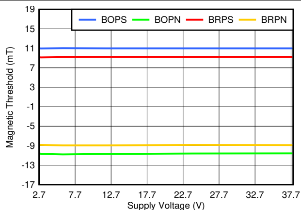
7-12. TMAG5123D Magnetic Thresholds vs. Voltage
