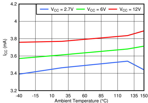
7-1. TMAG5123 I_{CC} vs. Temperature
