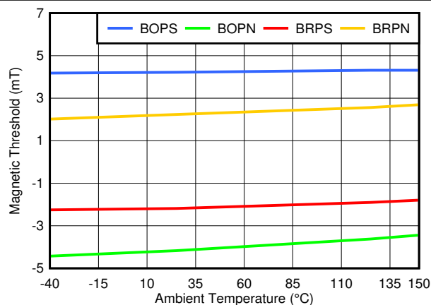
7-3. TMAG5123B Magnetic Thresholds vs. Temperature
