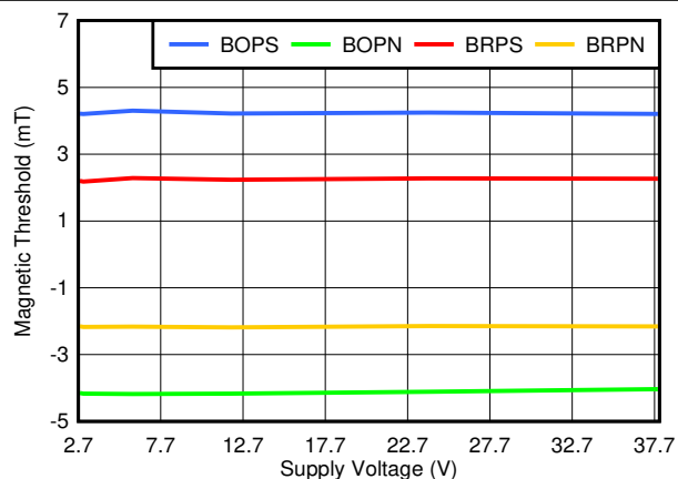
7-4. TMAG5123B Magnetic Thresholds vs. Voltage
