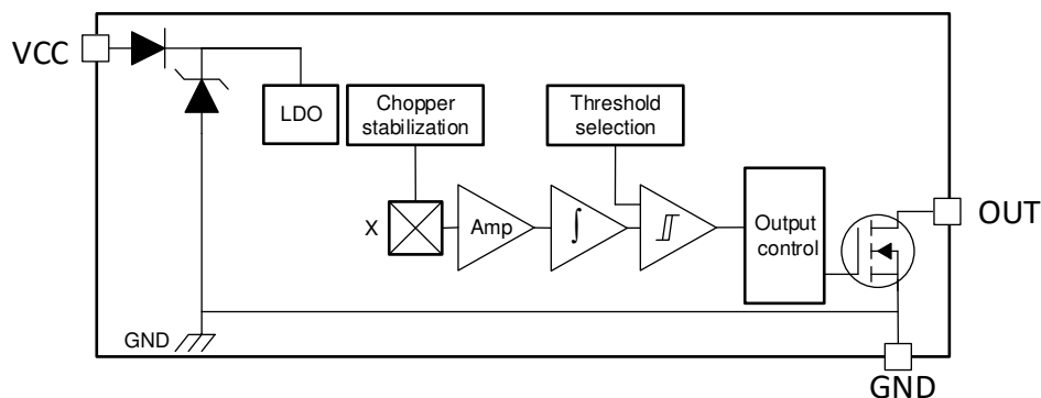
8-1. Block Diagram
