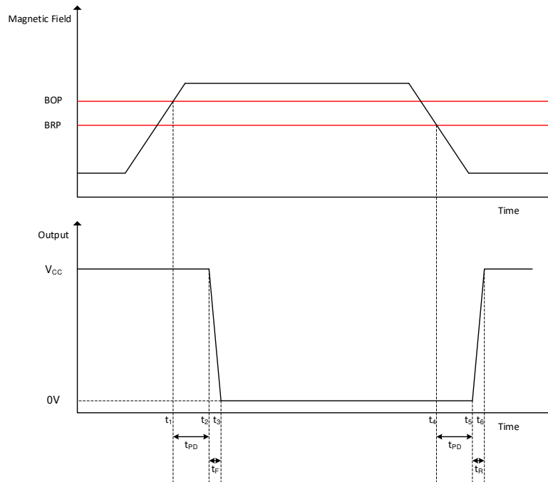
8-8. Propagation Delay
