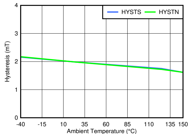
7-5. TMAG5123B Hysteresis vs. Temperature
