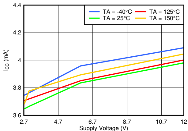
7-2. TMAG5123 I_{CC} vs. Voltage
