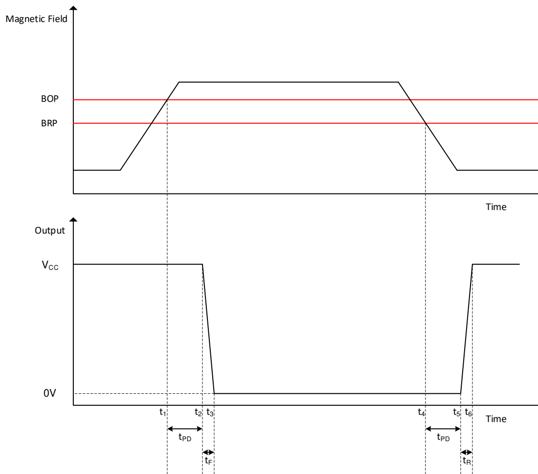
図 7-22. Propagation Delay
