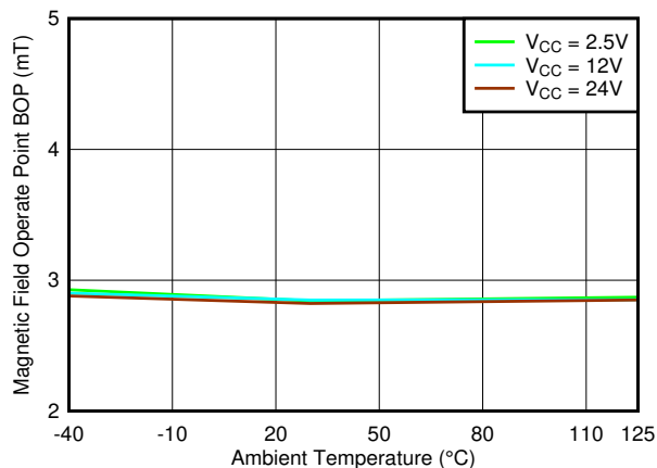
図 6-46. B OP_X Threshold vs Temperature
