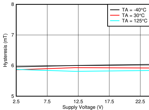
Figure 6-43. Hysteresis_Z vs V CC
