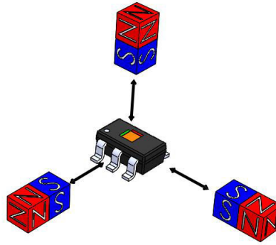
✎ 8-4. Axis Polarities
