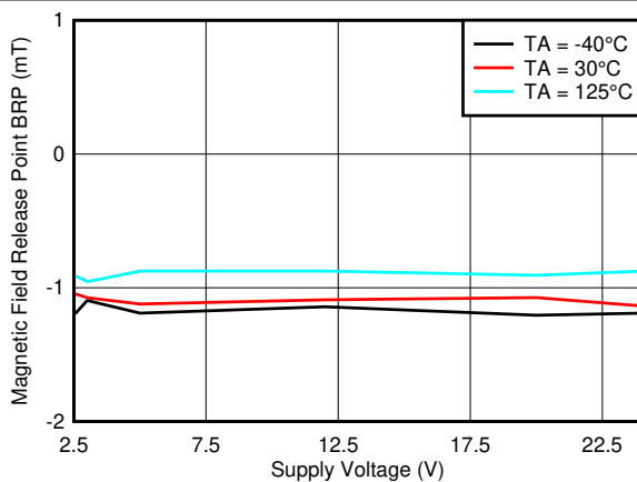
7-3. B_{RP\_Z} Threshold vs. V_{CC}
