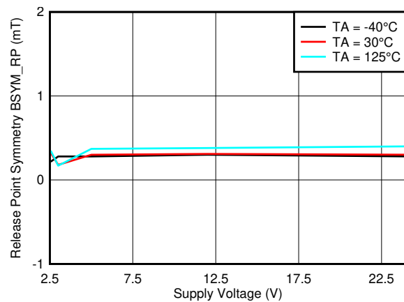
Figure 7-31. B_{SYM\_RP(ZY)} vs. V_{CC}
