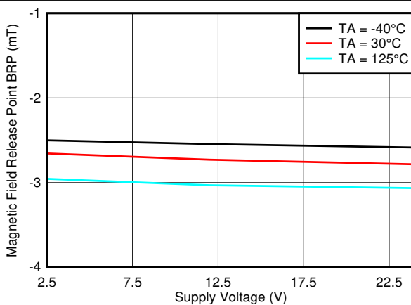
图 7-53. BRP_Y Threshold vs. VCC
