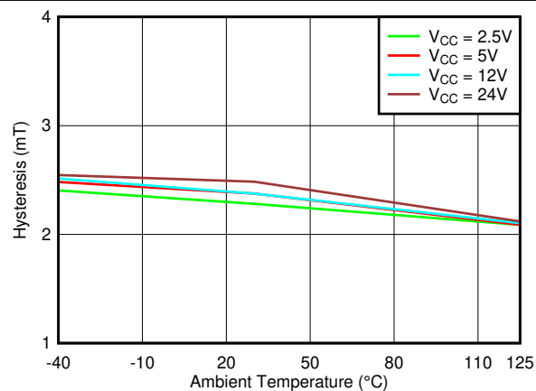
7-6. Hysteresis_Z vs. Temperature
