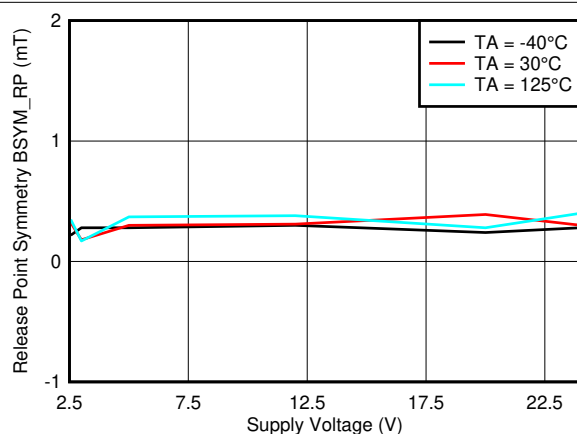
7-27. B_{SYM\_RP(ZX)} vs. V_{CC}
