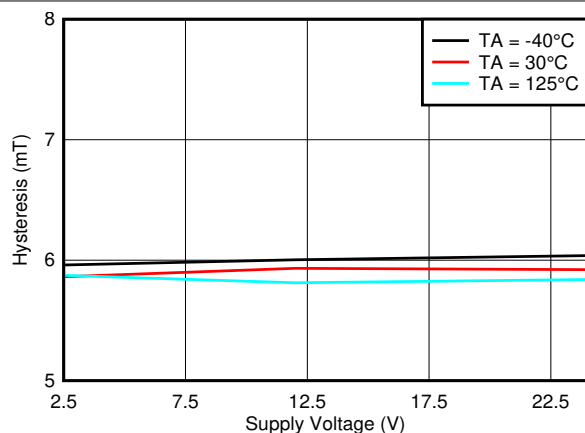
7-43. Hysteresis_Z vs. V CC
