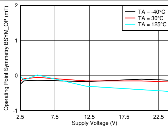
7-25. B_{SYM\_OP(ZX)} vs. V_{CC}
