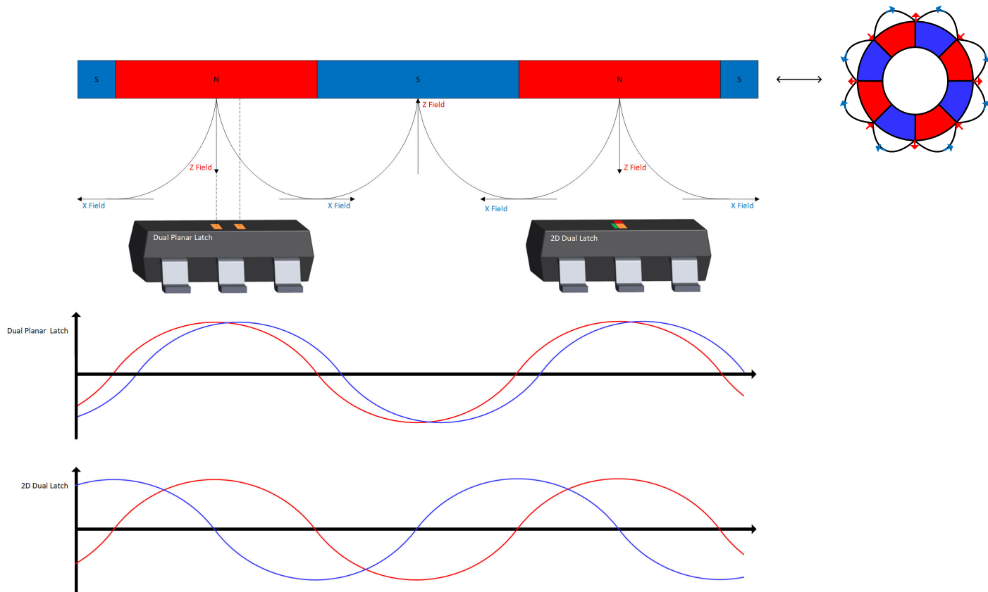
FIG 8-1. Dual Planar Latch vs. 2D Dual Latch
