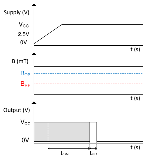
☒ 8-18. Power-On Time When B > B_{OP}
