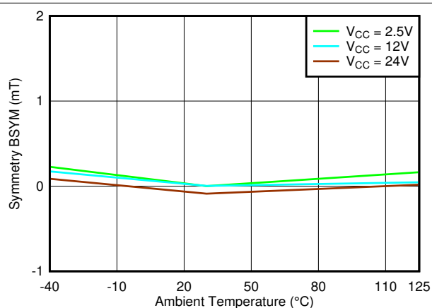
Figure 7-62. B_{SYM(Y)} vs. Temperature
