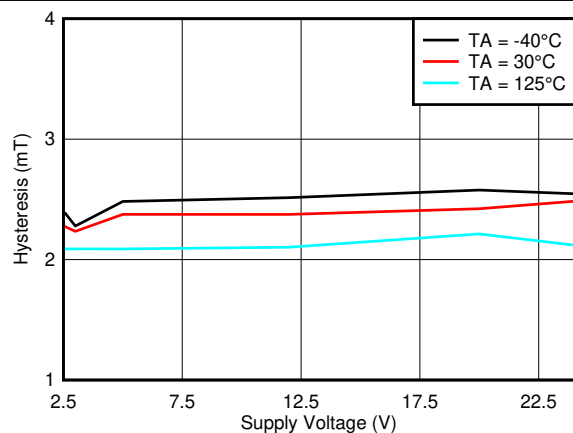
7-5. Hysteresis_Z vs. V_{CC}
