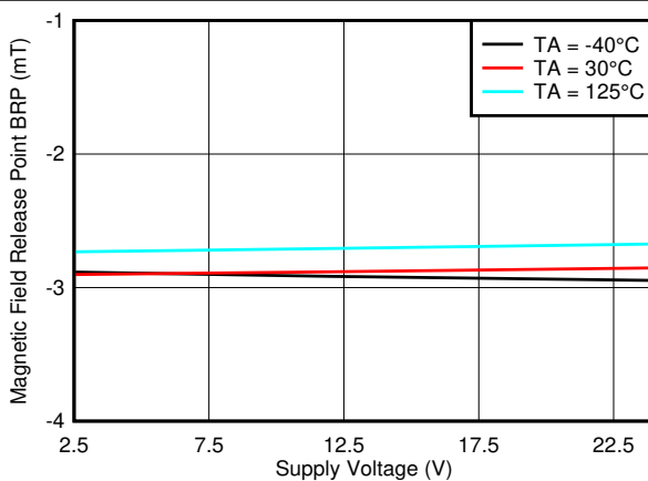
7-41. B RP_Z Threshold vs. V CC
