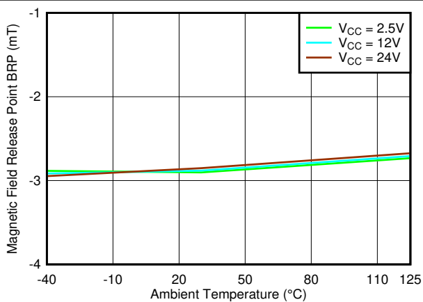
7-42. B RP_Z Threshold vs. Temperature
