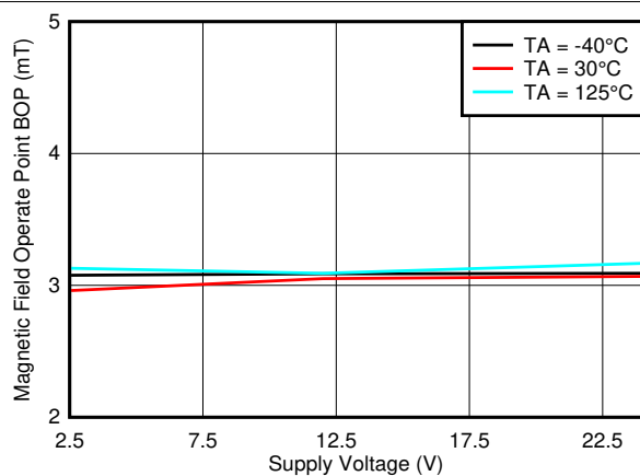
7-39. B OP_Z Threshold vs. V CC
