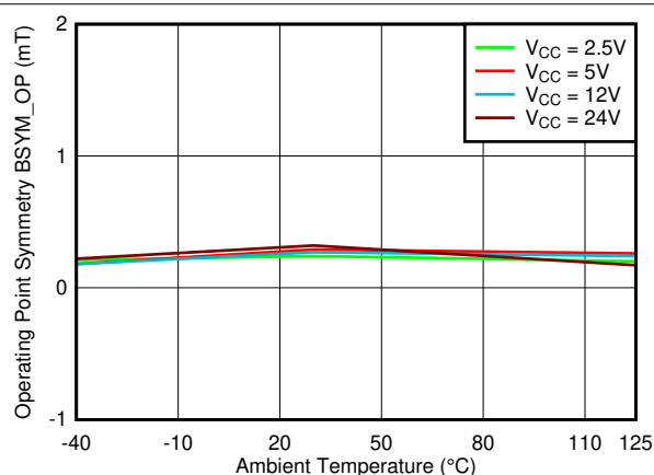
7-30. B_{SYM\_OP(ZY)} vs. Temperature
