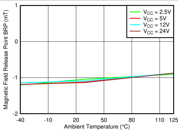
7-4. B_{RP\_Z} Threshold vs. Temperature
