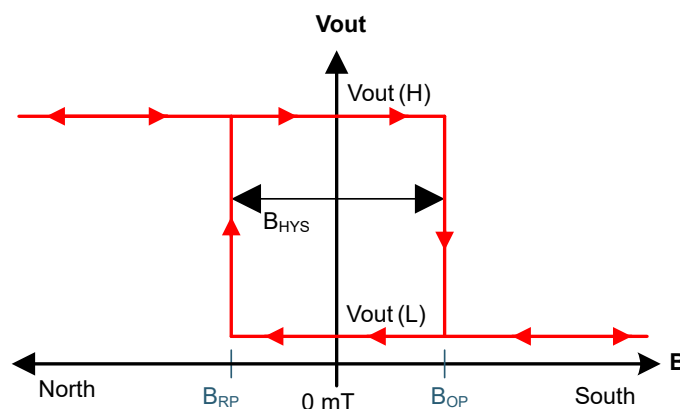
FIG 8-2. Latch Functionality
