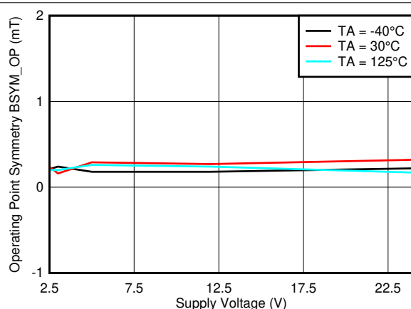
7-29. B_{SYM\_OP(ZY)} vs. V_{CC}
