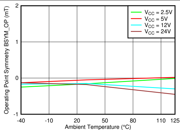
7-26. B_{SYM\_OP(ZX)} vs. Temperature
