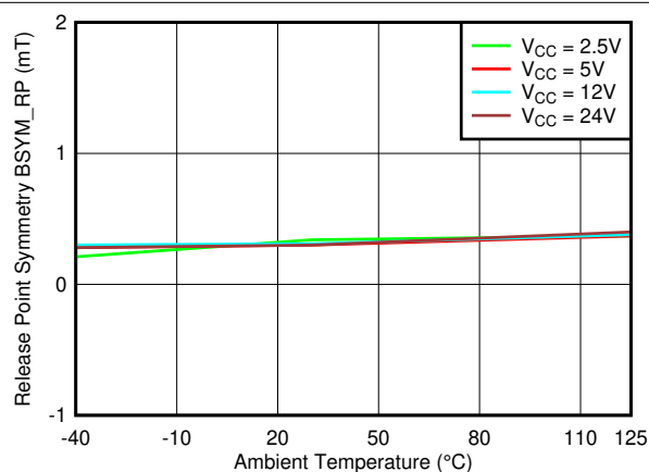
7-28. B_{SYM\_RP(ZX)} vs. Temperature
