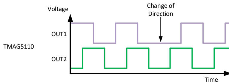
图 9-2. TMAG5110 Output Response
