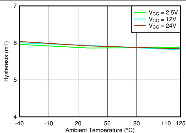
7-44. Hysteresis_Z vs. Temperature
