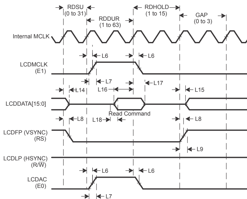
Figure 32-52. Command Read in Hitachi Mode
