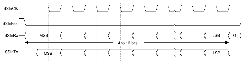
Figure 20-7. Freescale SPI Frame Format (Single Transfer) with SPO=1 and SPH=0
