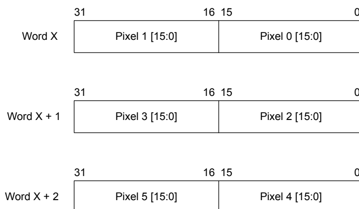
Figure 21-8. 16 bpp Data Format
