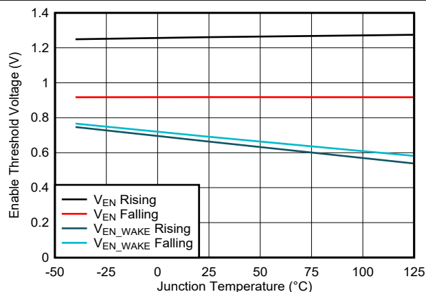
Figure 6-5. Enable Thresholds
