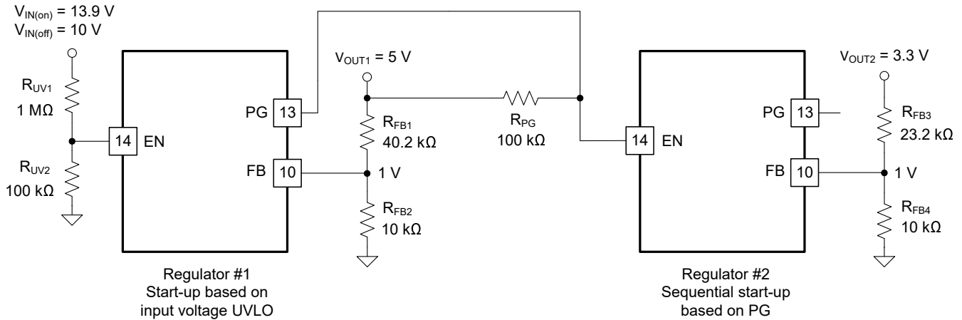
FIG 8-4. TLVM13620 Sequencing Implementation Using PG and EN
