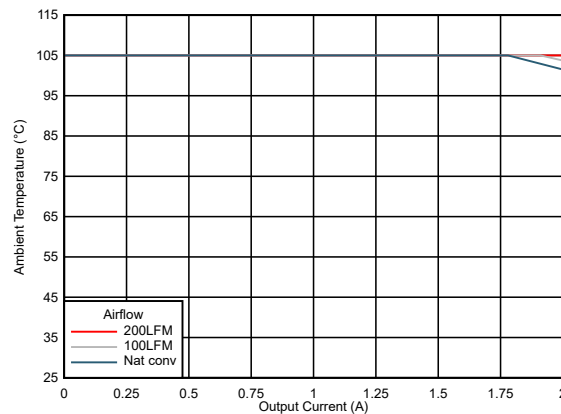
Figure 7-14. Safe Operating Area ( V_{OUT} = 3.3\text{ V} )
