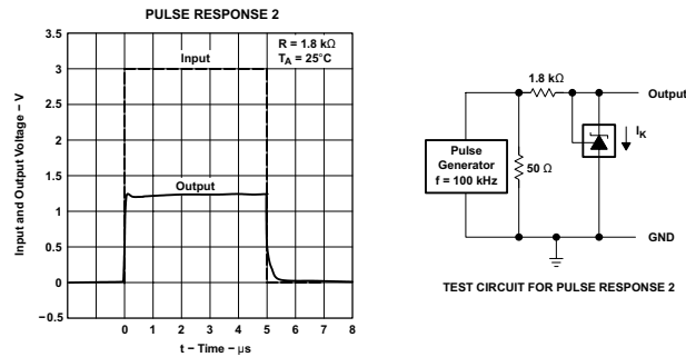
図 5-13. Pulse Response 2
