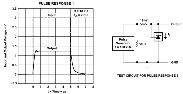
図 5-12. Pulse Response 1
