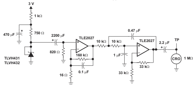
図 5-10. Equivalent Input Noise Voltage
