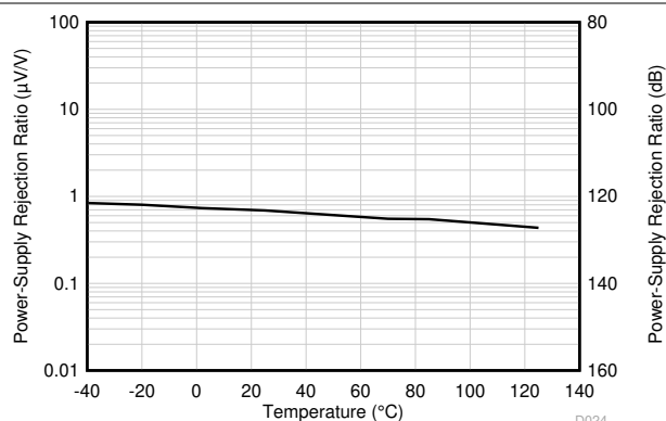
FIG 5-19. PSRR vs Temperature
