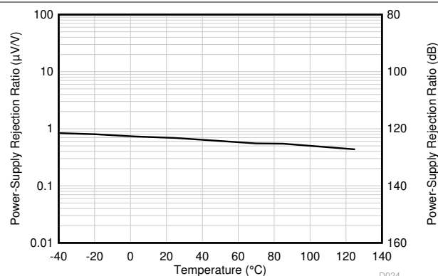
FIG 5-19. PSRR vs Temperature
