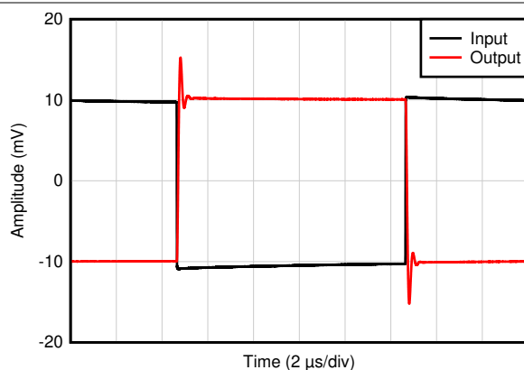
C_L = 20\text{pF} , G = -1 , 20\text{mV}_{pp} step response
