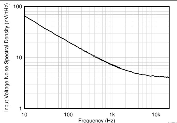
FIG 5-21. Input Voltage Noise Spectral Density vs Frequency
