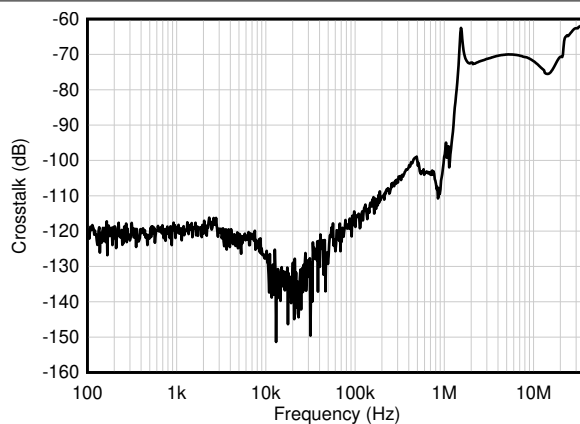
5-36. Channel Separation vs Frequency
