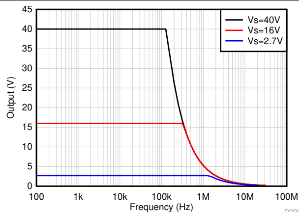
5-35. Maximum Output Voltage vs Frequency
