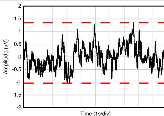
FIG 5-20. 0.1Hz to 10-Hz Noise
