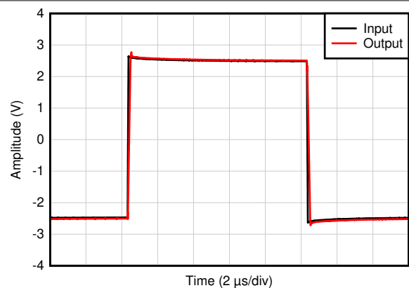
C_L = 20\text{pF} , G = 1 , 5\text{V}_{pp} step response
