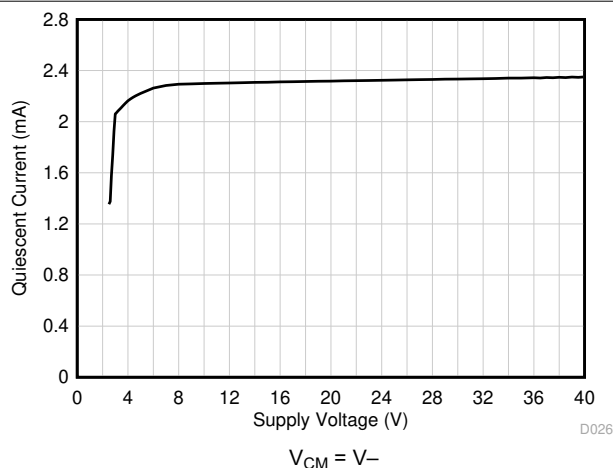
FIG 5-22. Quiescent Current vs Supply Voltage
