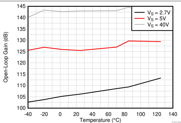
FIG 5-24. Open-Loop Voltage Gain vs Temperature (dB)
