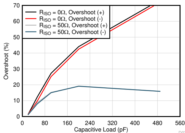
図 6-3. Small-Signal Overshoot vs Capacitive Load (20mV pp Output Step, G = +1 )
