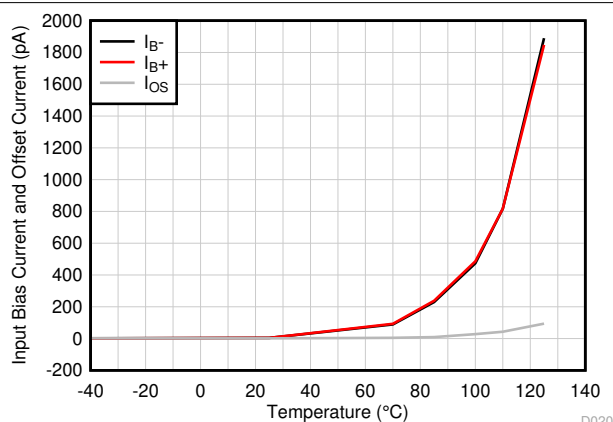
Figure 5-10. Input Bias Current and Offset Current vs Temperature
