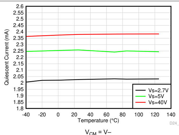
FIG 5-23. Quiescent Current vs Temperature
