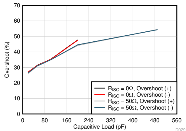
図 6-4. Small-Signal Overshoot vs Capacitive Load (20mV pp Output Step, G = -1 )
