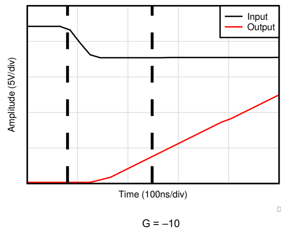
6-30. Negative Overload Recovery
