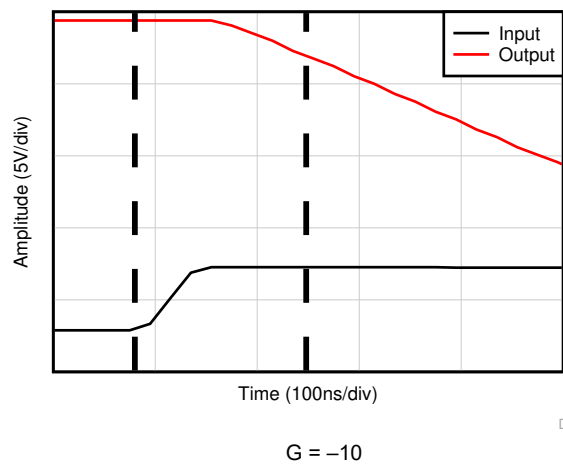
6-29. Positive Overload Recovery
