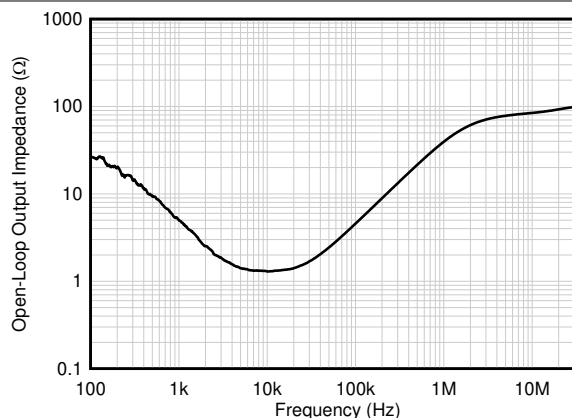
図 5-30. Open-Loop Output Impedance vs Frequency
