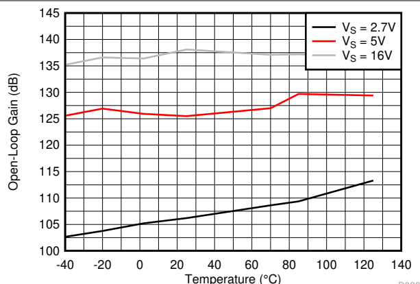
図 5-29. Open-Loop Voltage Gain vs Temperature (dB)
