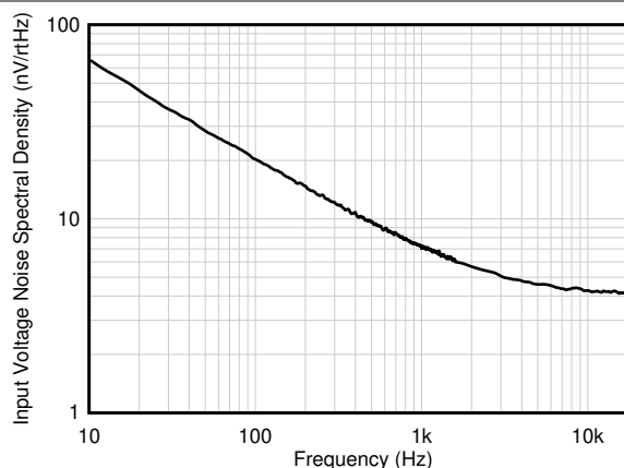
図 5-26. Input Voltage Noise Spectral Density vs Frequency
