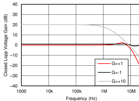
図 5-8. Closed-Loop Gain vs Frequency
