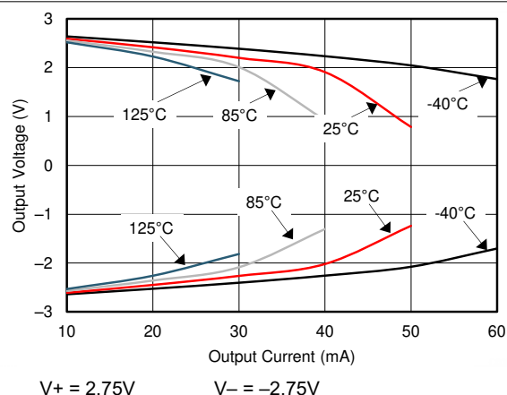
図 5-10. Output Voltage Swing vs Output Current
