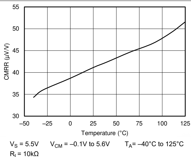
図 5-12. CMRR vs Temperature
