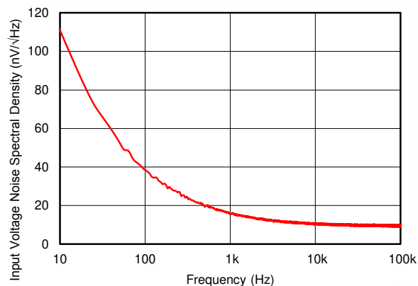
図 5-16. Input Voltage Noise Spectral Density vs Frequency
