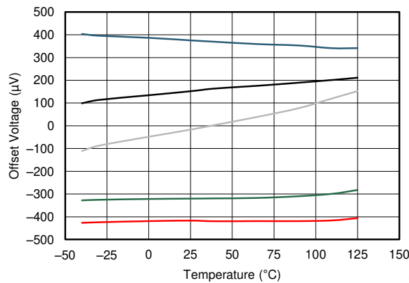
FIG 5-3. Offset Voltage vs Temperature
