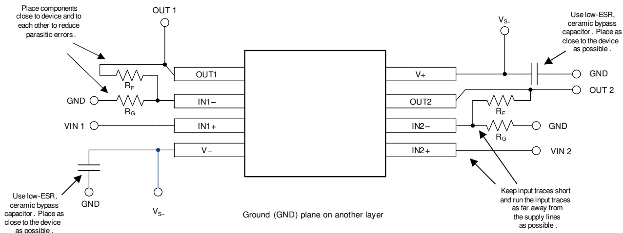
7-5. Layout Example
