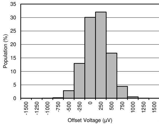
FIG 5-1. Offset Voltage Production Distribution
