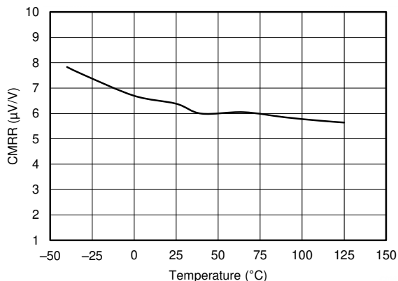
図 5-13. CMRR vs Temperature
