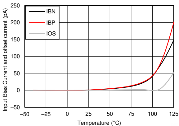
図 5-9. Input Bias Current vs Temperature
