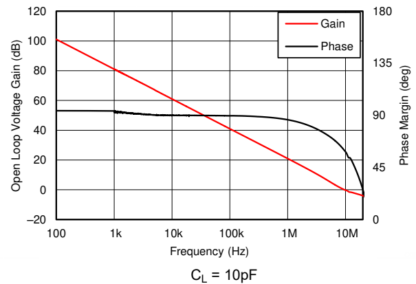
FIG 5-6. Open-Loop Gain and Phase vs Frequency
