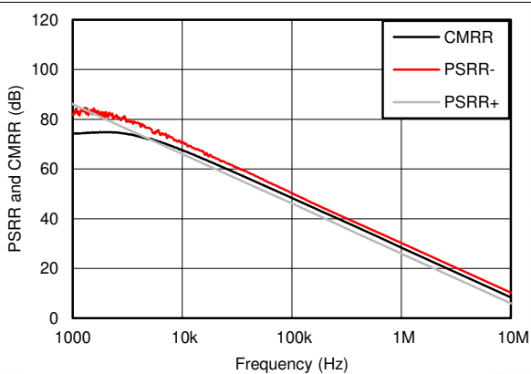
図 5-11. CMRR and PSRR vs Frequency (Referred to Input)
