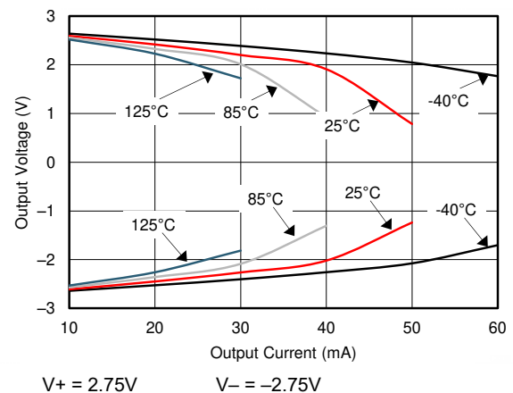
図 5-10. Output Voltage Swing vs Output Current
