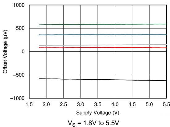
FIG 5-5. Offset Voltage vs Power Supply
