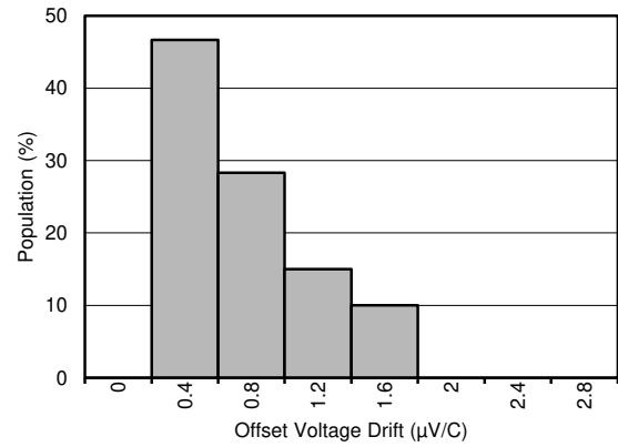
FIG 5-2. Offset Voltage Drift Distribution
