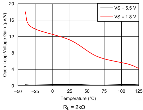
図 5-7. Open-Loop Gain vs Temperature
