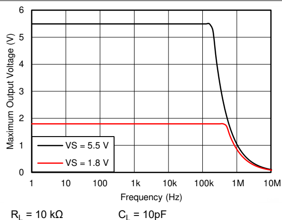
5-30. Maximum Output Voltage vs Frequency and Supply Voltage
