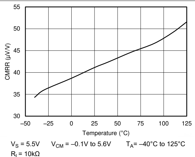
図 5-12. CMRR vs Temperature
