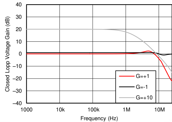
図 5-8. Closed-Loop Gain vs Frequency
