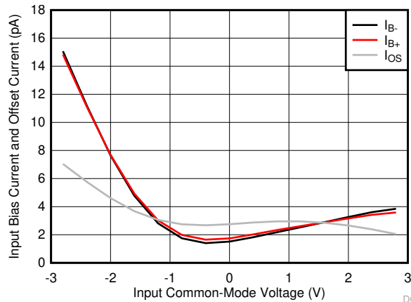
图 6-7. Input Bias Current and Offset Current vs Common-Mode Voltage
