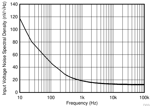
5-9. Input Voltage Noise Spectral Density vs Frequency
