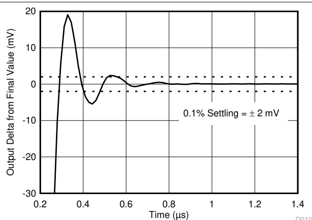
Figure 5-25. Large-Signal Step Response
