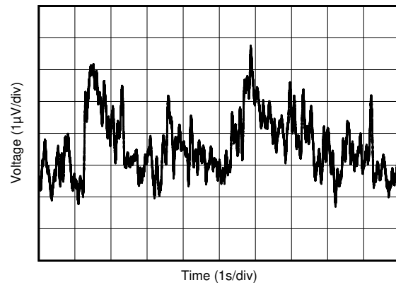
5-8. 0.1Hz to 10Hz Input Voltage Noise
