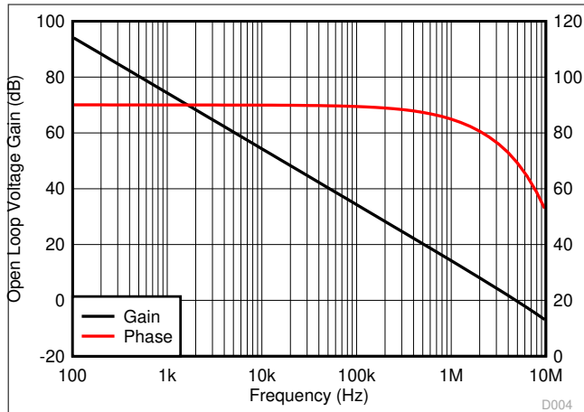
5-13. Open Loop Voltage Gain and Phase vs Frequency
