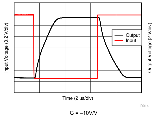
5-22. Overload Recovery
