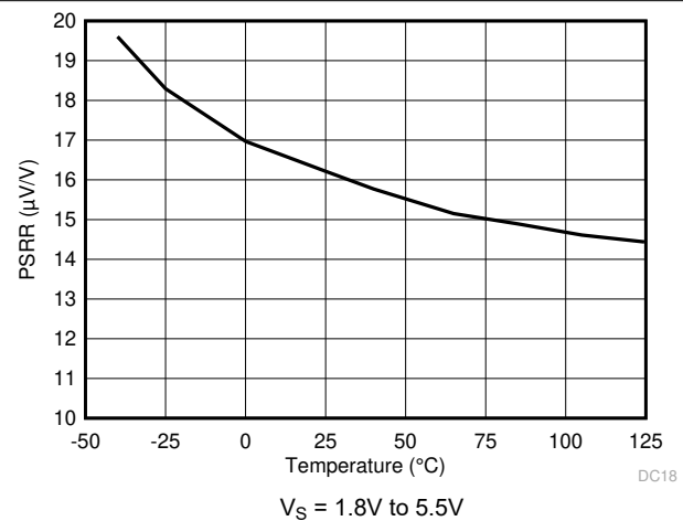
5-12. PSRR vs Temperature
