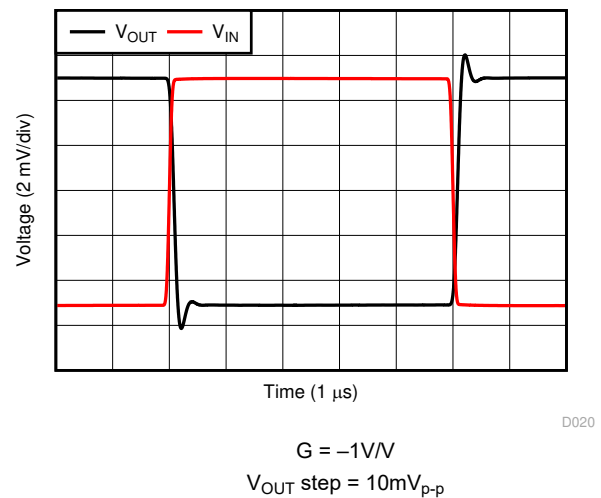
5-24. Small-Signal Step Response
