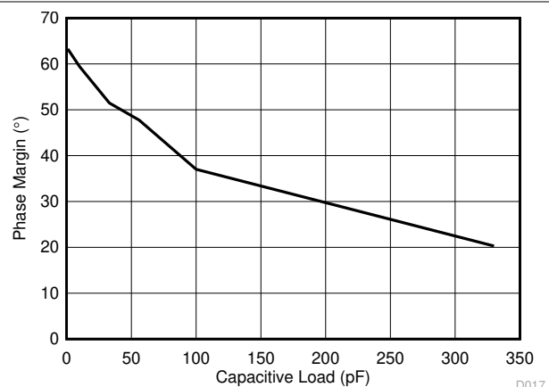
5-17. Phase Margin vs Capacitive Load
