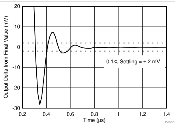
Figure 5-26. Large-Signal Step Response
