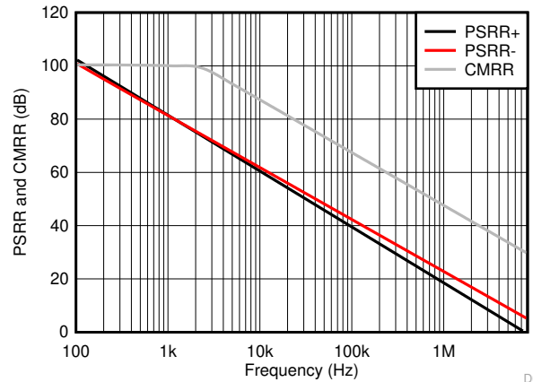
5-10. CMRR and PSRR vs Frequency (Referred to Input)
