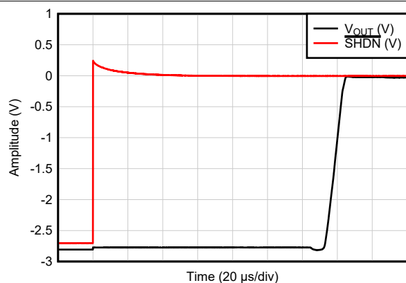
FIG 7-43. Amplifier Enable Response
