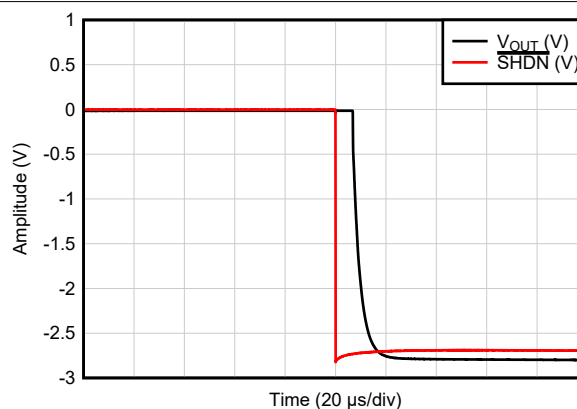
FIG 7-44. Amplifier Disable Response
