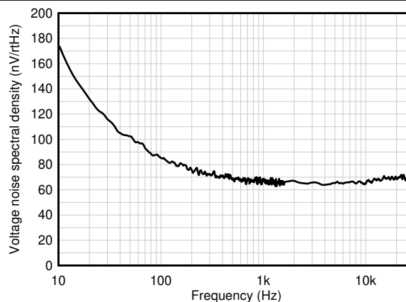
7-22. Input Voltage Noise Spectral Density
