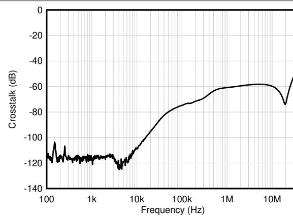
FIG 7-46. Channel Separation
