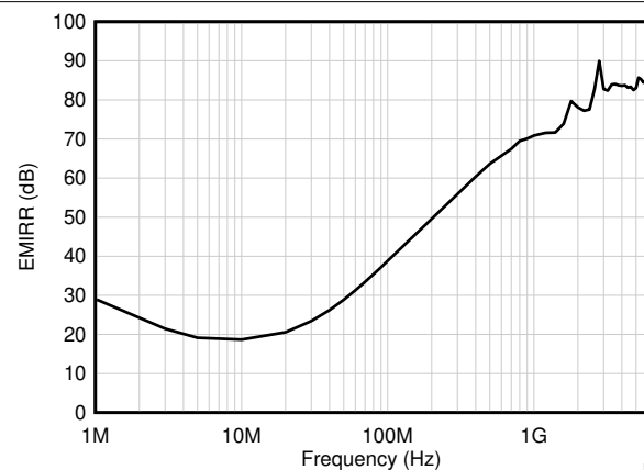
FIG 7-45. Electromagnetic Interference Rejection Ratio Referred to Noninverting Input (EMIRR+) vs Frequency
