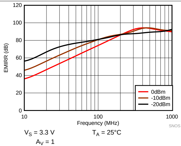
Figure 25. EMIRR Performance
