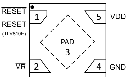
Figure 6-5. DPW Package 5-Pin X2SON See Table 6-1 Top View
