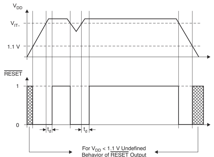
7-1. Timing Diagram
