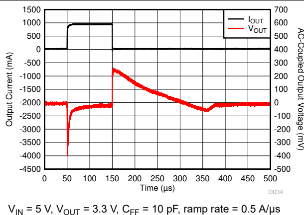
6-11. I_{OUT} Transient From 1\text{ mA} to 1\text{ A}
