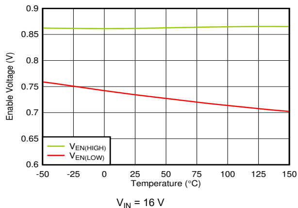
FIG 6-24. V_{EN} Thresholds vs Temperature
