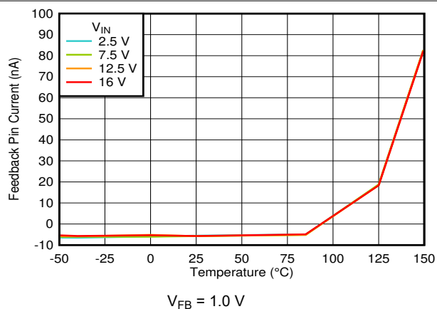
6-32. I_{FB} vs Temperature
