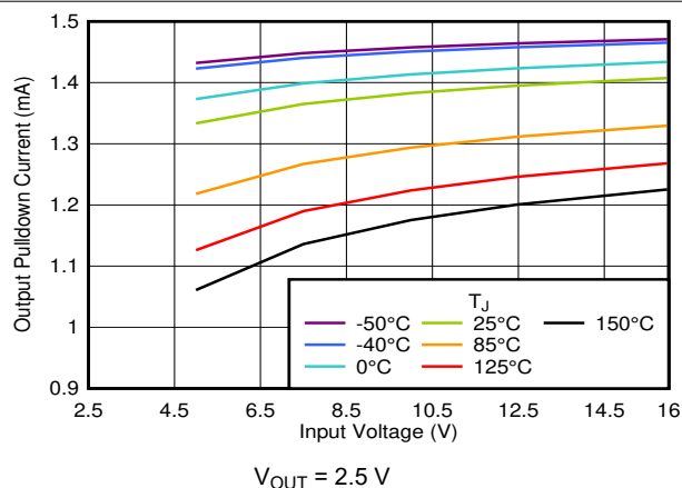
6-31. I_{PULLDOWN} vs V_{IN}
