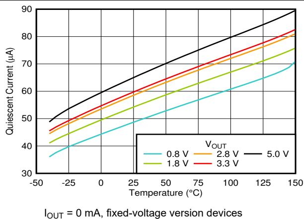
FIG 6-6. I_Q vs Temperature
