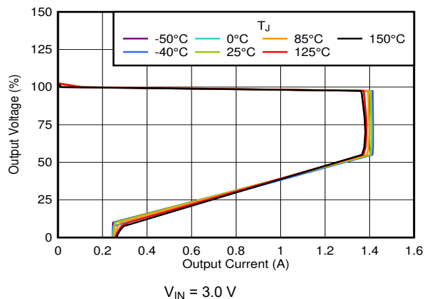
FIG 6-19. Foldback Current Limit vs I_{OUT} and Temperature
