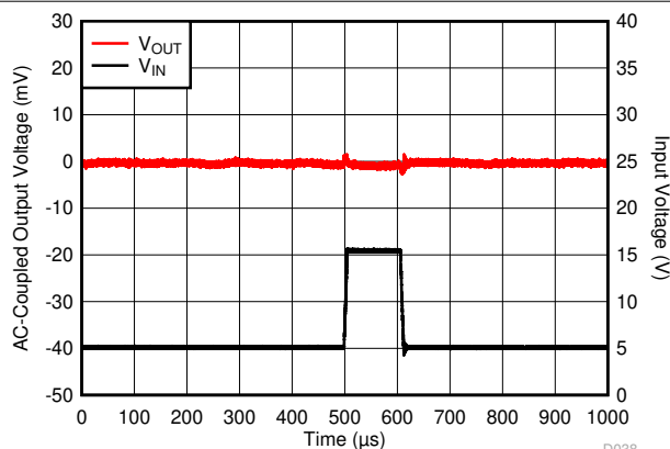
FIG 6-14. V_{IN} Transient From 5 V to 16 V
