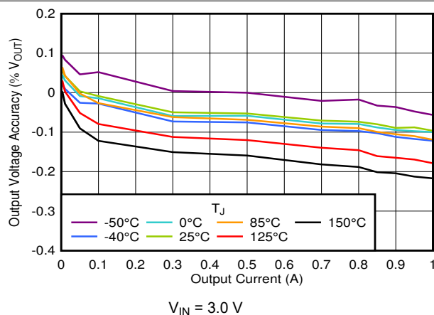
FIG 6-1. V_{OUT} Accuracy vs I_{OUT}
