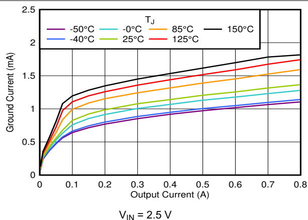
6-8. I_{GND} vs I_{OUT}
