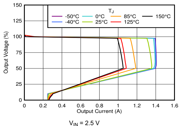
FIG 6-20. Foldback Current Limit vs I_{OUT} and Temperature
