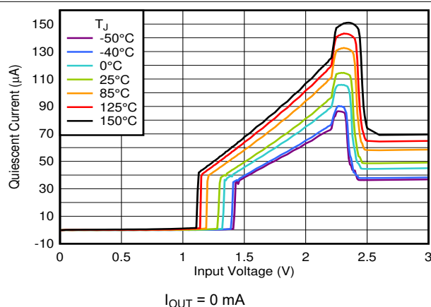
6-9. I_Q Increase Below Minimum V_{IN}
