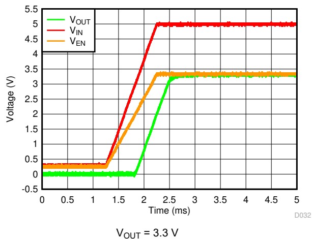
FIG 6-21. Startup With Separate V_{EN} and V_{IN}
