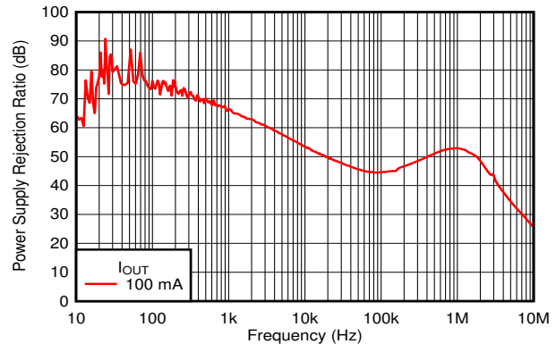
8-4. PSRR Performance
