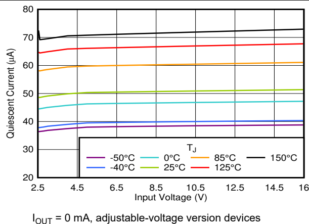
FIG 6-5. I_Q vs V_{IN}
