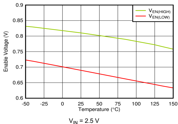
FIG 6-23. V_{EN} Thresholds vs Temperature
