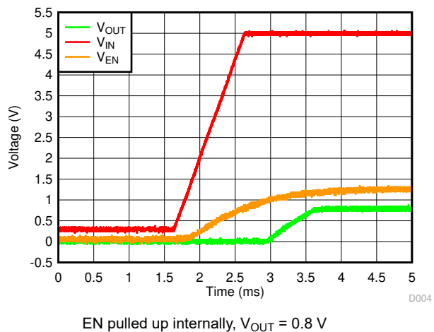
FIG 6-22. Startup With V_{EN} Floating
