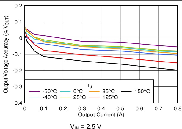
FIG 6-2. V_{OUT} Accuracy vs I_{OUT}
