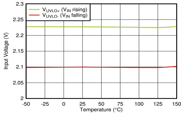
6-25. UVLO Thresholds vs Temperature
