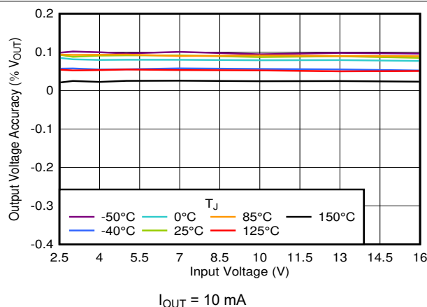
FIG 6-3. V_{OUT} Accuracy vs V_{IN}
