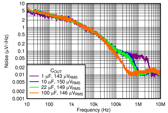
V_{OUT} = 3.3\text{V} , V_{RMS} BW = 10Hz to 100kHz 5-4. Output Spectral Noise Density vs Frequency and C_{OUT}
