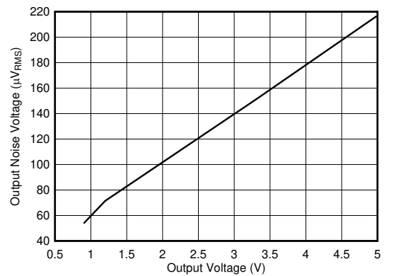
I_{OUT} = 500\text{mA} , C_{OUT} = 1\mu\text{F} , V_{RMS} BW = 10Hz to 100kHz 5-6. Output Noise Voltage vs V_{OUT}
