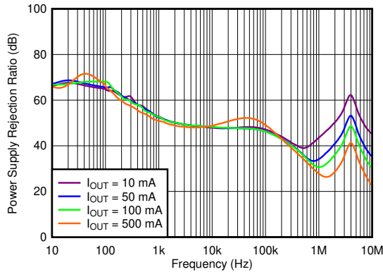
V_{IN} = 4.3\text{V} , V_{OUT} = 3.3\text{V} , C_{OUT} = 1\mu\text{F} 5-1. PSRR vs Frequency and I_{OUT}
