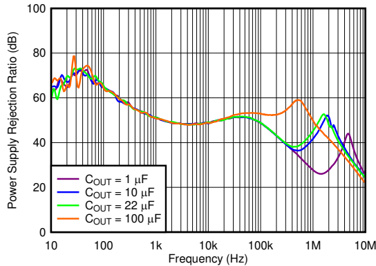
V_{IN} = 4.3\text{V} , V_{OUT} = 3.3\text{V} , I_{OUT} = 500\text{mA} 5-3. PSRR vs Frequency and C_{OUT}
