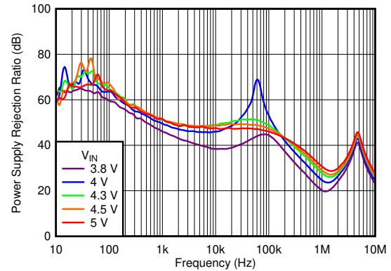
V_{OUT} = 3.3\text{V} , C_{OUT} = 1\mu\text{F} , I_{OUT} = 500\text{mA} 5-2. PSRR vs Frequency and V_{IN}
