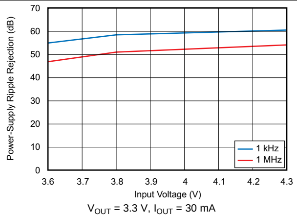
FIG 26. Power-Supply Ripple Rejection vs Input Voltage
