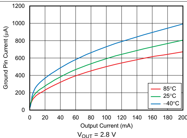
FIG 17. Ground Pin Current vs Output Current
