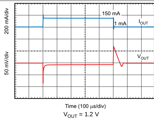
FIG 30. Load Transient Response
