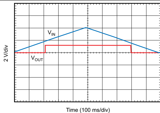
FIG 39. Line Transient Response
