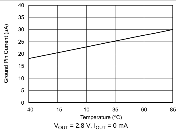
FIG 15. Ground Pin Current vs Temperature
