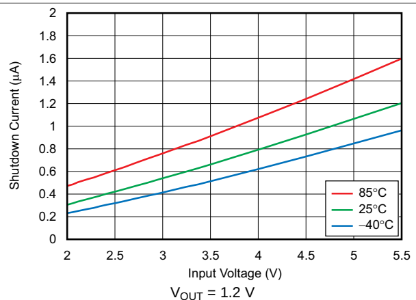
FIG 18. Shutdown Current vs Input Voltage
