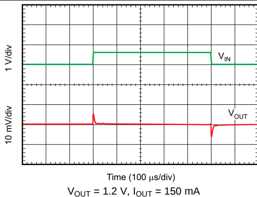
FIG 33. Line Transient Response
