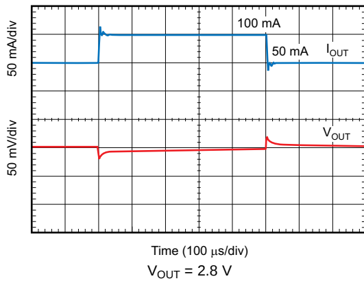
FIG 31. Load Transient Response
