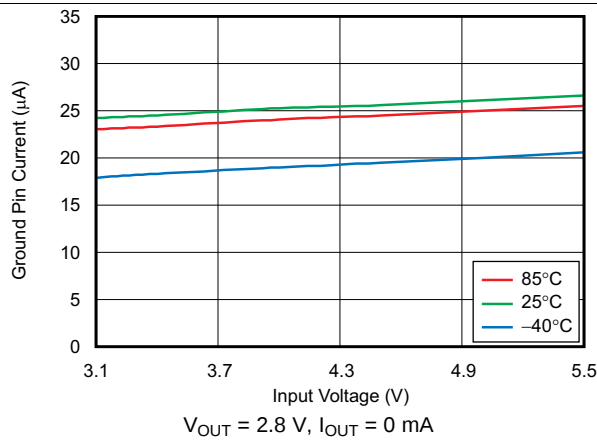
FIG 13. Ground Pin Current vs Input Voltage
