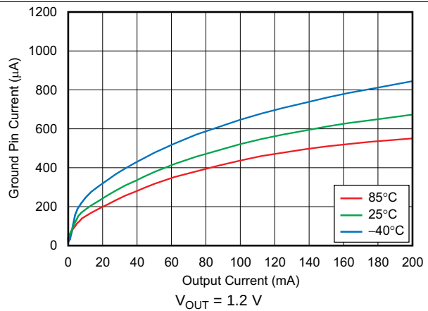
FIG 16. Ground Pin Current vs Output Current
