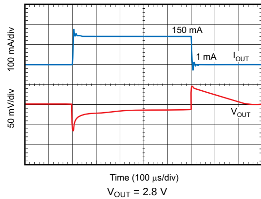
FIG 32. Load Transient Response
