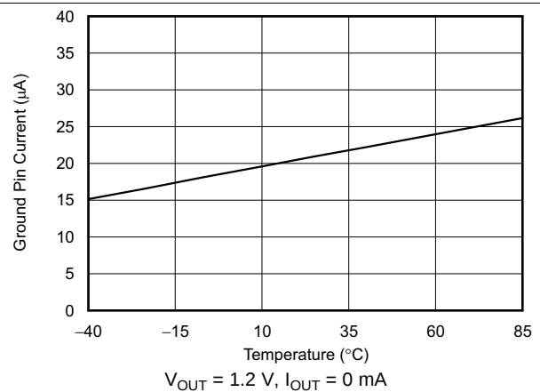
FIG 14. Ground Pin Current vs Temperature
