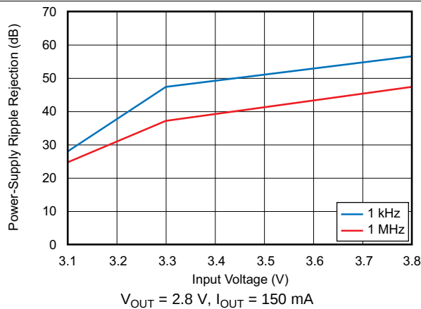
FIG 25. Power-Supply Ripple Rejection vs Input Voltage
