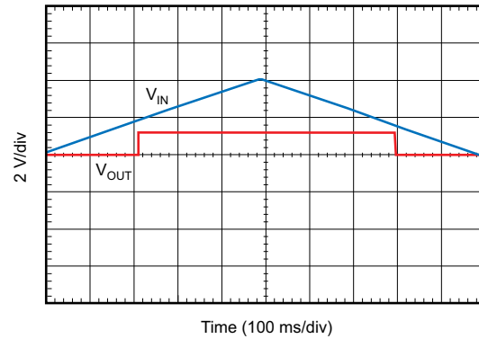
52. V_{IN} Ramp Up, Ramp Down Response
