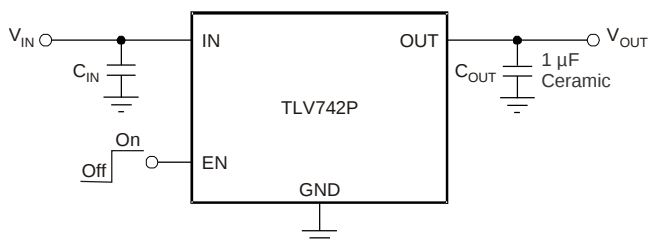
図 44. Typical Application Circuit
