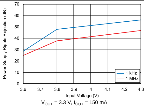
FIG 27. Power-Supply Ripple Rejection vs Input Voltage
