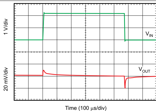
FIG 37. Line Transient Response
