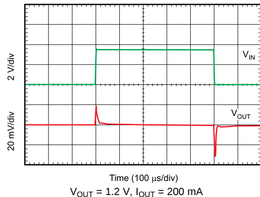
FIG 36. Line Transient Response
