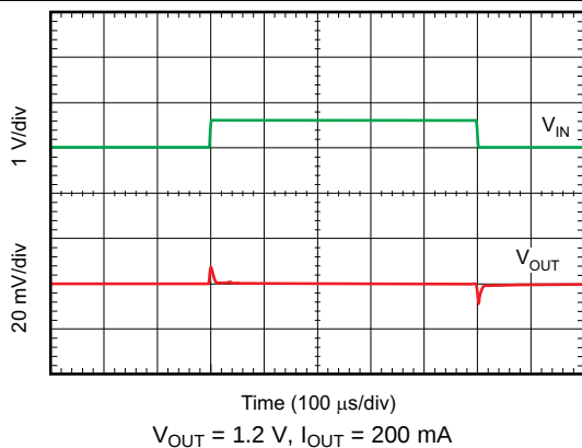
Figure 49. Line Transient Response
