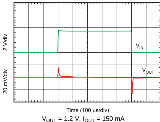
FIG 35. Line Transient Response
