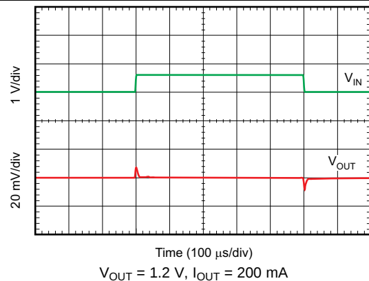
FIG 34. Line Transient Response
