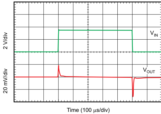
51. Line Transient Response
