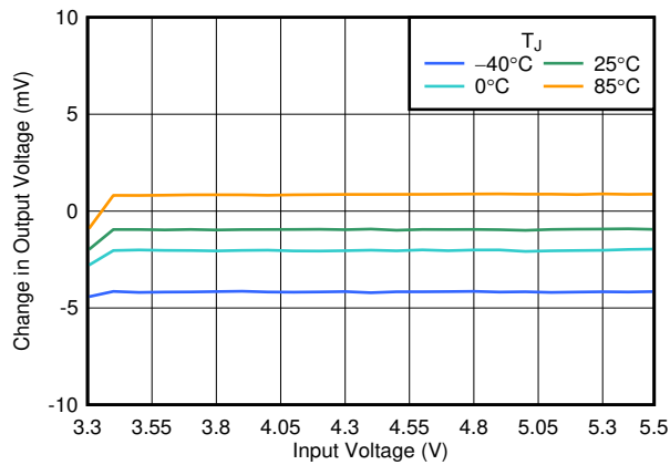
FIG 6-1. Line Regulation vs V_{IN}
