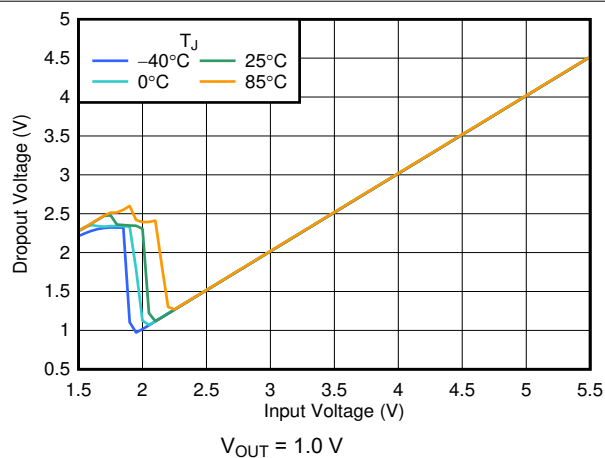
FIG 6-5. Dropout Voltage vs V_{IN}
