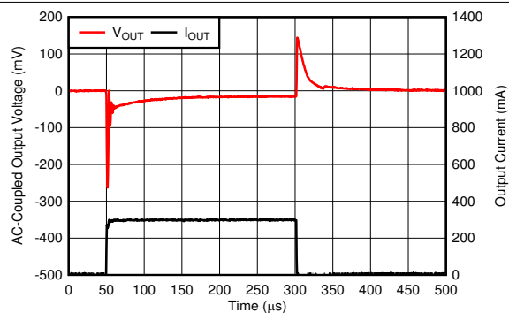
Figure 6-21. Load Transient
