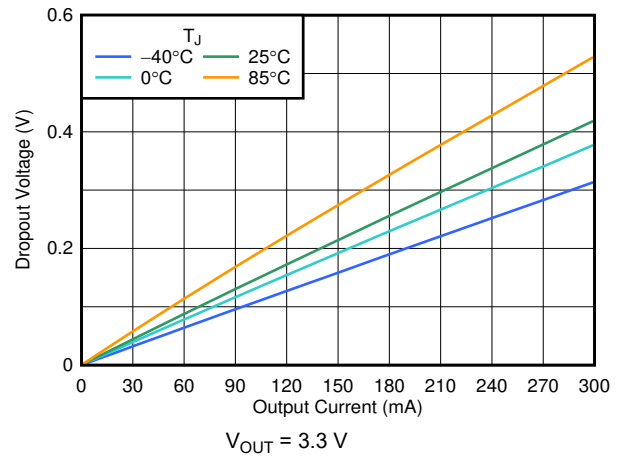
FIG 6-4. Dropout Voltage vs I_{OUT}
