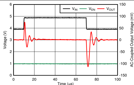
Figure 6-20. Line Transient
