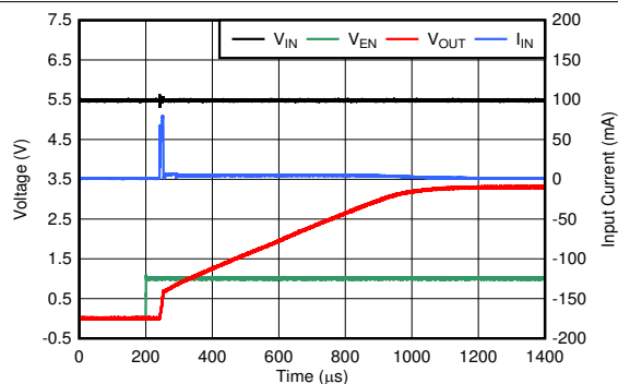
FIG 6-25. Start-Up With EN, Inrush Current
