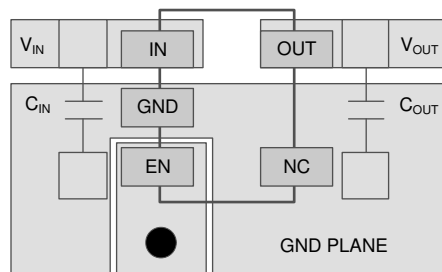
✎ 10-1. Layout Example for the DQN Package
