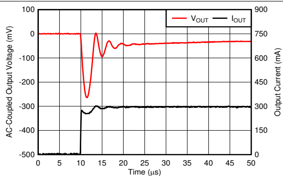
Figure 6-22. Load Transient
