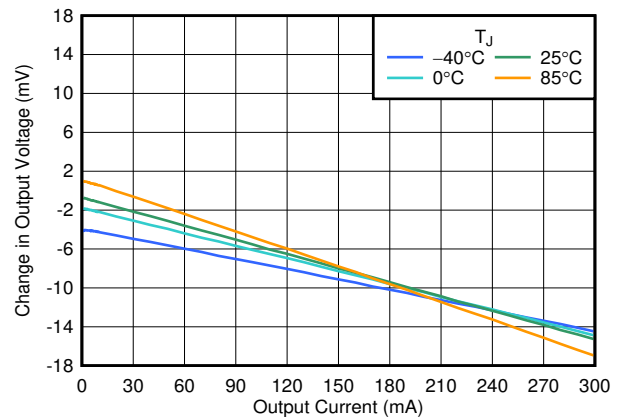
FIG 6-2. Load Regulation vs I_{OUT}
