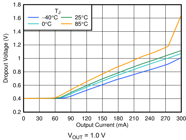
FIG 6-3. Dropout Voltage vs I_{OUT}
