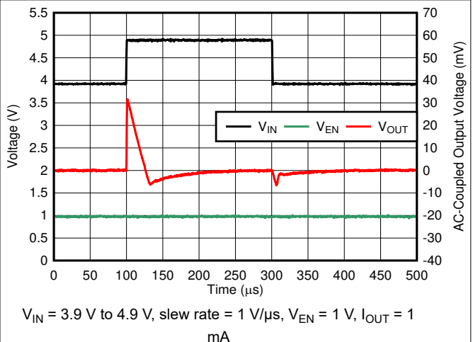
6-18. Line Transient
