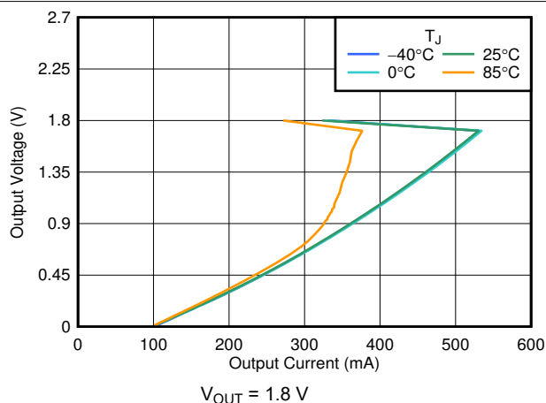
6-8. Foldback Current Limit vs I_{OUT}
