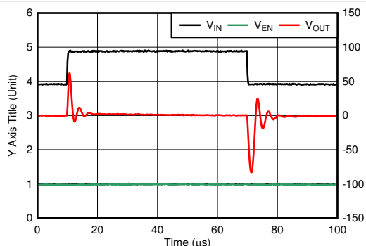
Figure 6-19. Line Transient
