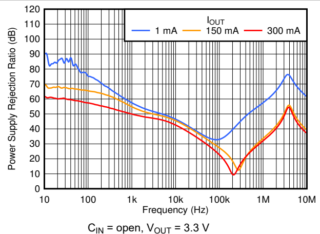
6-16. PSRR vs Frequency and I_{OUT}
