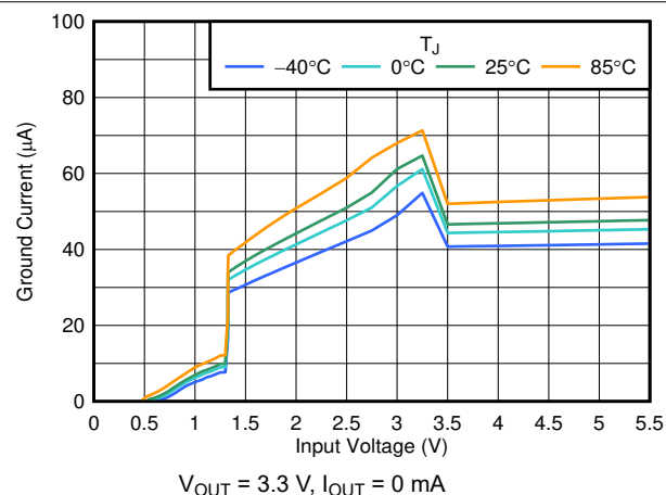
6-10. I_{GND} vs V_{IN}
