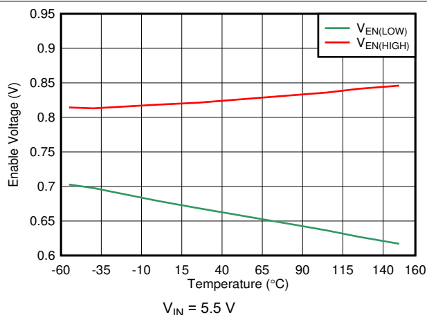
6-12. EN High and Low Threshold vs Temperature
