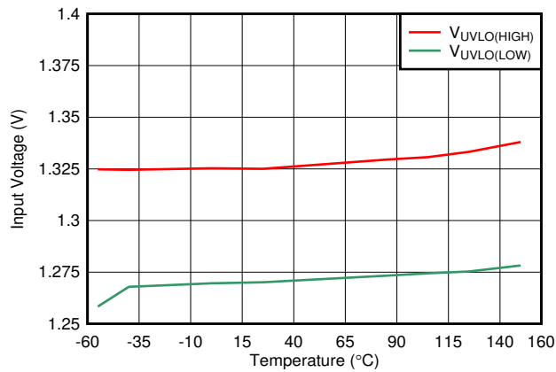
6-13. UVLO Rising and Falling Threshold vs Temperature
