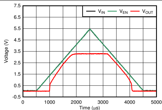
FIG 6-26. Start-Up and Shutdown
