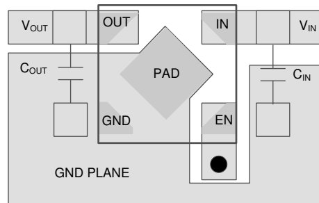
✎ 10-1. Layout Example for the DQN Package
