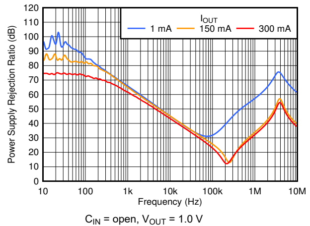
6-14. PSRR vs Frequency and I_{OUT}
