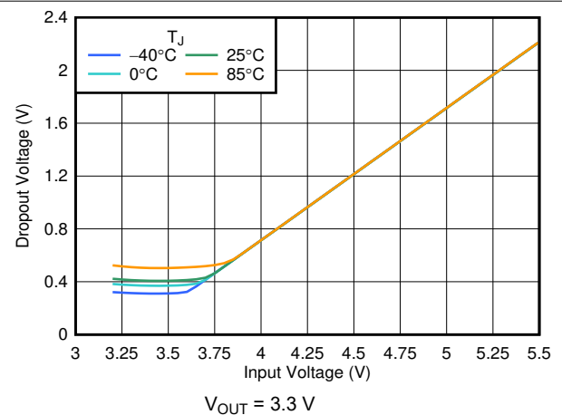
FIG 6-6. Dropout Voltage vs V_{IN}
