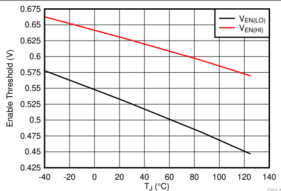
FIG 6-5. Enable Threshold vs Temperature
