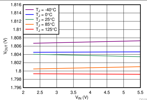
FIG 6-1. 1.8-V Regulation vs V_{IN} (Line Regulation) and Temperature
