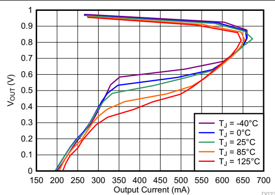
FIG 6-6. Output Voltage vs 1.0-V Foldback Current Limit and Temperature
