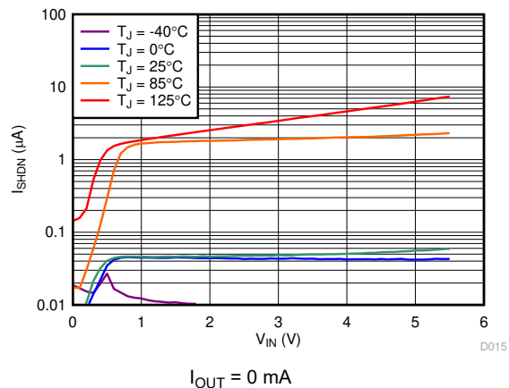
FIG 6-4. Shutdown Current vs V_{IN} and Temperature
