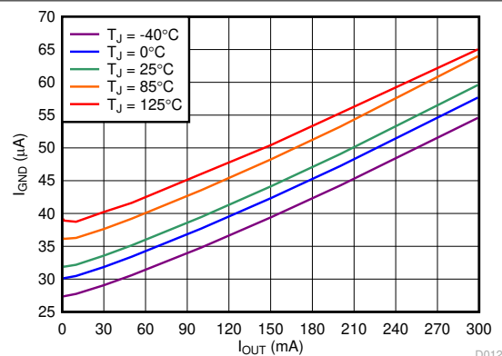
FIG 6-2. Ground Pin Current vs I_{OUT} and Temperature
