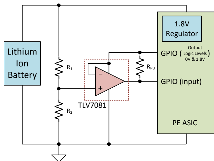
Figure 23. Battery Monitor
