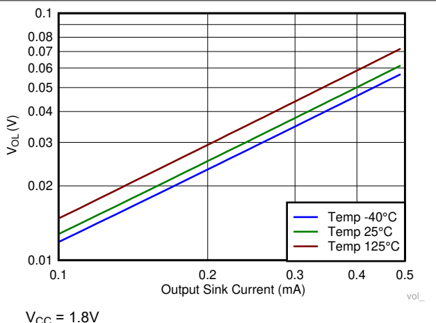
図 5-20. Output Voltage Low vs Output Sink Current
