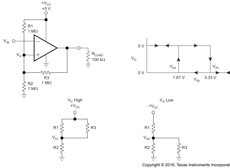
図 7-1. TLV703x in an Inverting Configuration With Hysteresis
