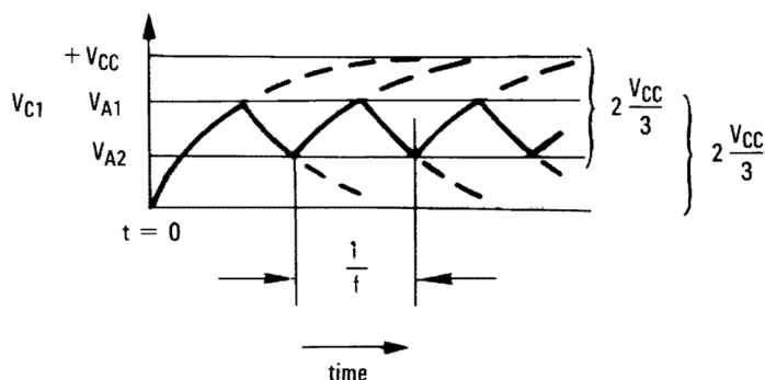
✎ 45. Square-Wave Oscillator Timing Thresholds
