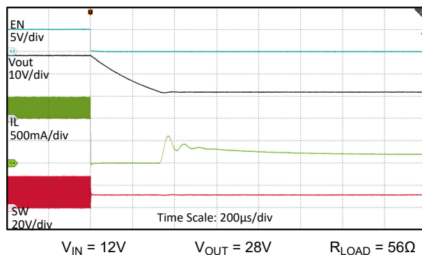
図 8-12. Shutdown by EN Waveforms
