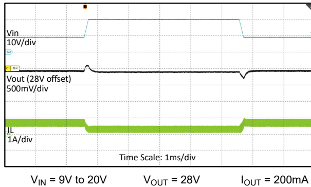
8-17. Line Transient
