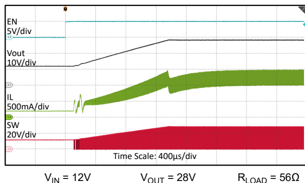
図 8-11. Start-up by EN Waveforms
