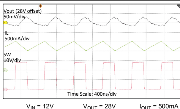
図 8-14. Switching Waveforms in Steady State
