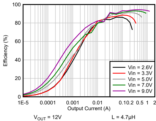
Figure 6-1. Efficiency vs Output Current, V_{OUT} = 12\text{V}
