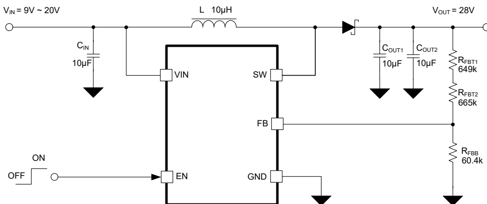
図 8-10. Typical 28V Application
