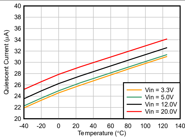
Figure 6-5. Quiescent Current vs Temperature
