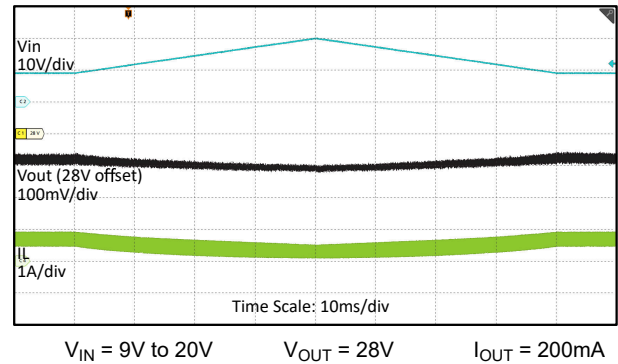
8-18. Line Sweep
