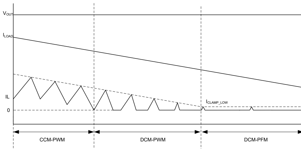
図 7-1. TLV61047 Functional Modes
