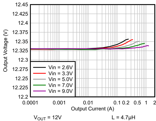
Figure 6-3. Load regulation, V_{OUT} = 12\text{V}
