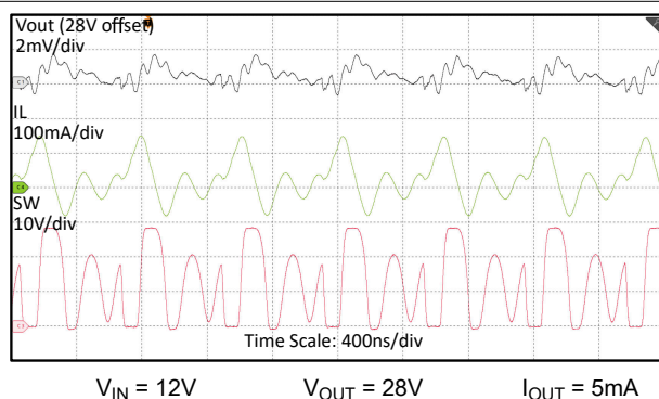
図 8-13. Switching Waveforms in Steady State
