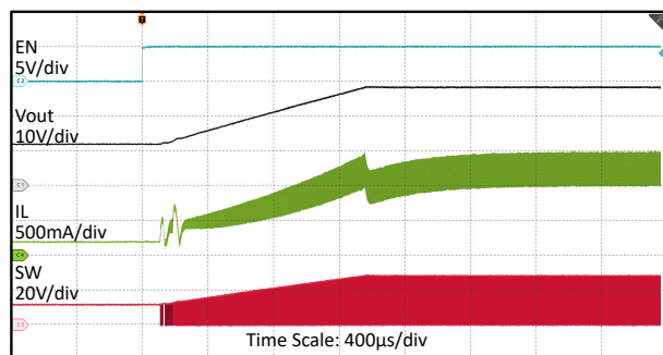
8-11. Start-up by EN Waveforms
