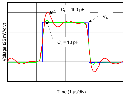
FIG 13. Small-Signal Pulse Response (Minimum Supply)
