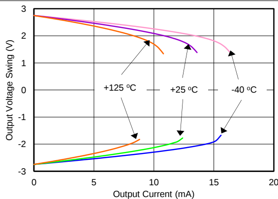
FIG 11. Output Voltage Swing vs Output Current
