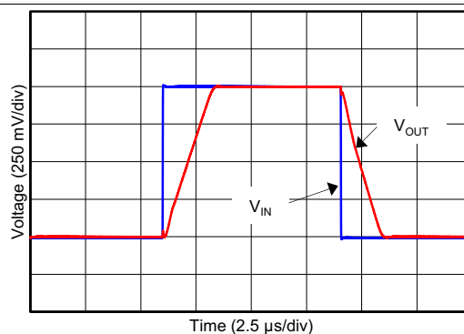
FIG 14. Small-Signal Pulse Response (Maximum Supply)
