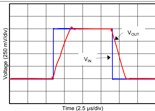
FIG 13. Small-Signal Pulse Response (Minimum Supply)
