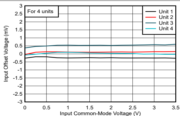
FIG 6-20. Offset Voltage vs. Common-Mode at 125°C, 5V
