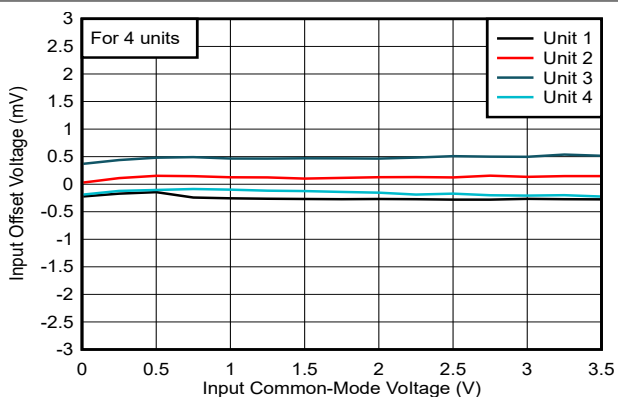
FIG 6-21. Offset Voltage vs. Common-Mode at 25°C, 5V
