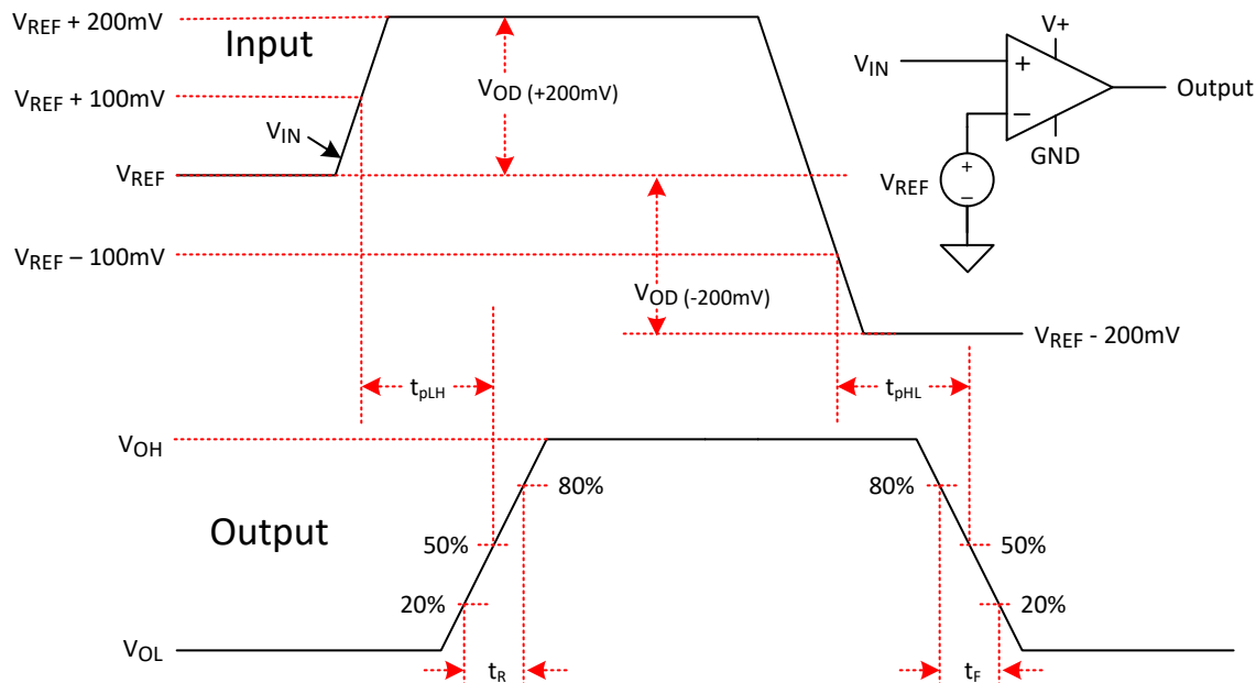
8-1. Comparator Timing Diagram
