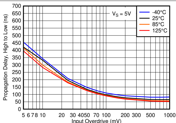
Figure 6-18. Propagation Delay, High to Low, 5V
