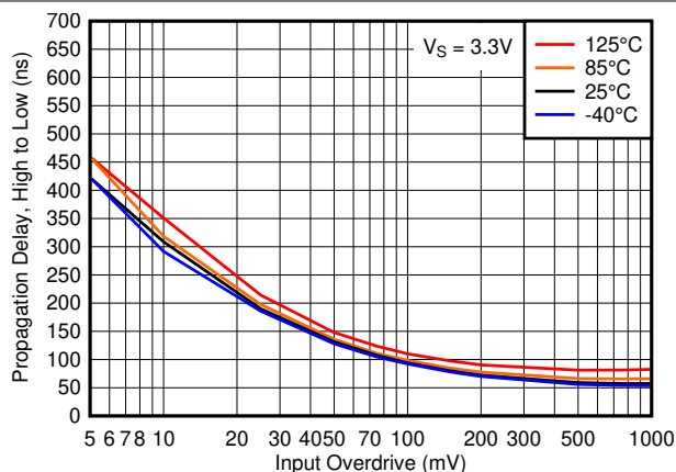
Figure 6-16. Propagation Delay, High to Low, 3.3V
