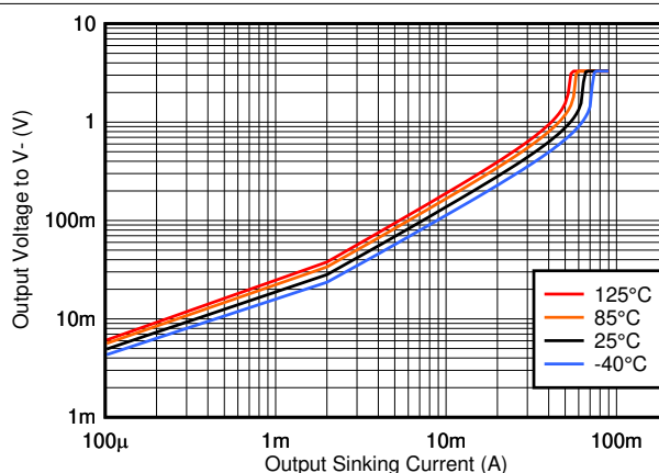
Figure 6-6. Output Sinking Current vs. Output Voltage, 3.3V
