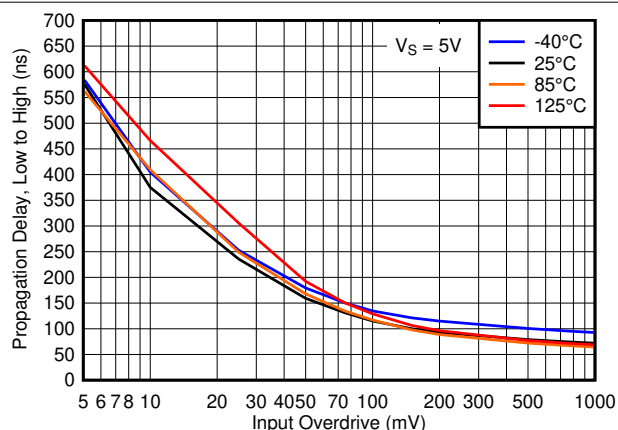
FIG 6-19. Propagation Delay, Low to High, 5V
