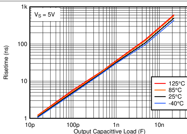
Figure 6-12. Risettime vs. Capacitive Load
