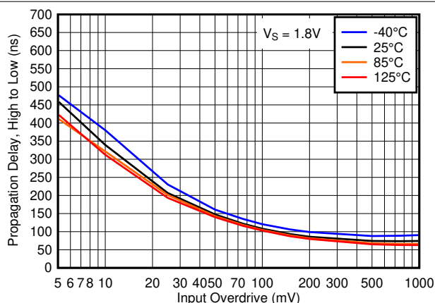
Figure 6-14. Propagation Delay, High to Low, 1.8V
