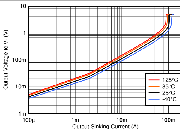
Figure 6-8. Output Sinking Current vs. Output Voltage, 5V
