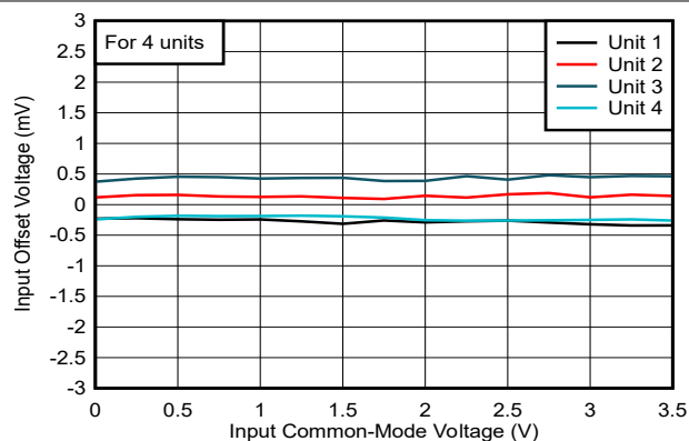
FIG 6-22. Offset Voltage vs. Common-Mode at -40°C, 5V
