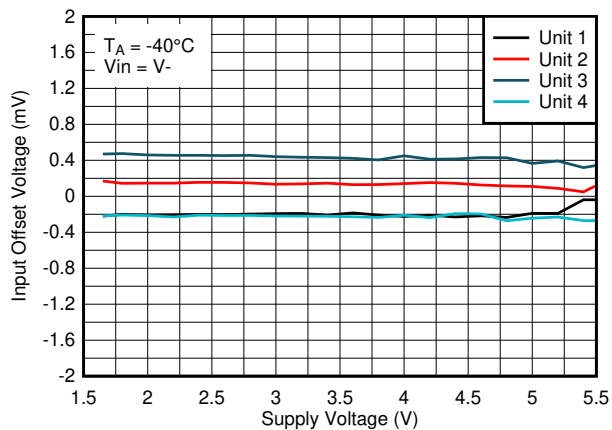
図 6-25. Offset Voltage vs. Supply Voltage at -40^\circ\text{C} , V_{\text{IN}} = V_-
