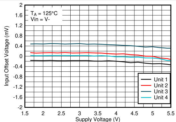
FIG 6-23. Offset Voltage vs. Supply Voltage at 125°C, V_{\text{IN}}=V_-
