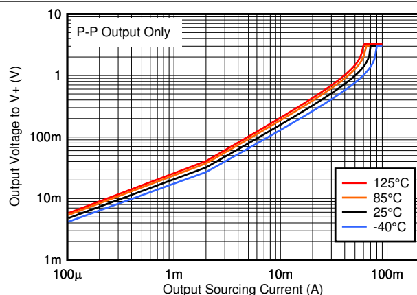
Figure 6-7. Output Sourcing Current vs. Output Voltage, 3.3V
