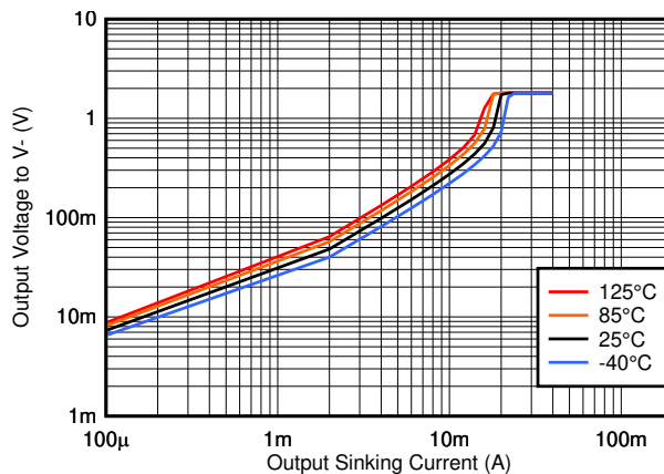
Figure 6-4. Output Sinking Current vs. Output Voltage, 1.8V
