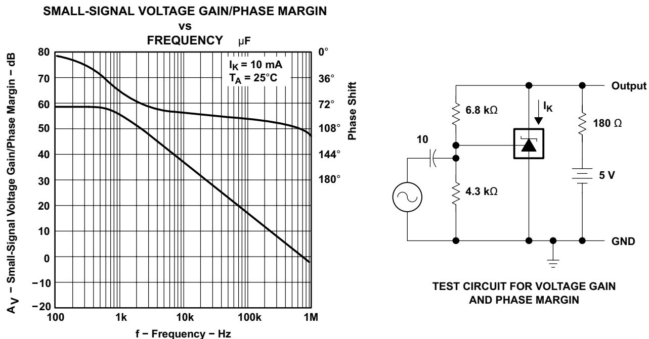
図 5-14. Voltage Gain and Phase Margin
