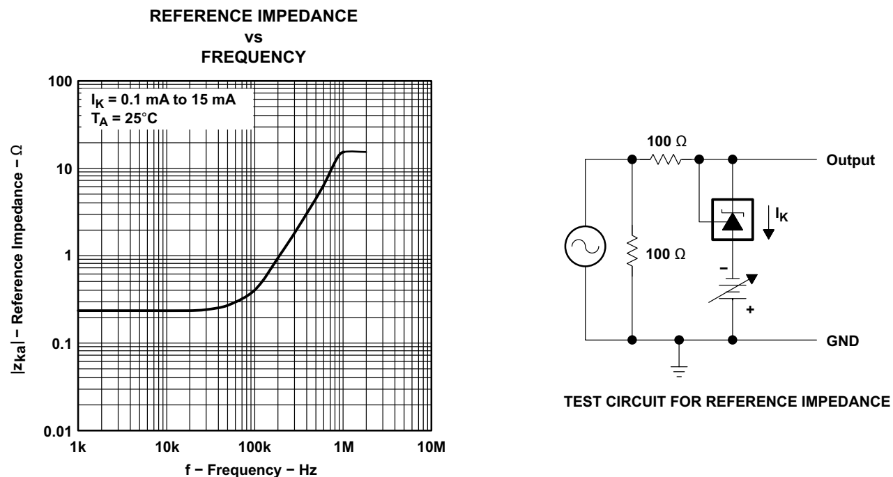
図 5-15. Reference Impedance vs Frequency
