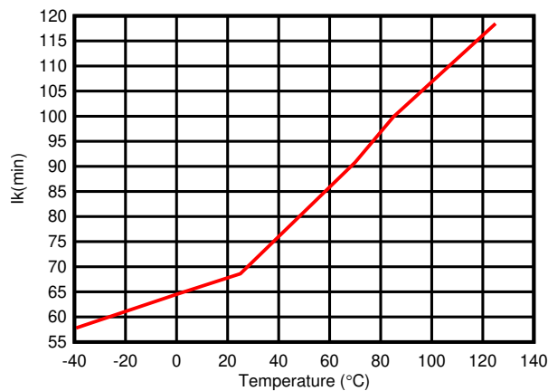
図 5-5. Minimum Cathode Current (μA) vs Temperature
