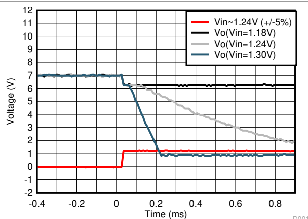
8-3. Output Response with Small Overdrive Voltages
