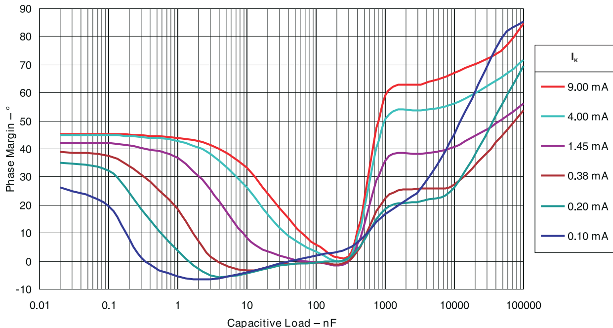
図 5-18. Stability Boundary Conditions
