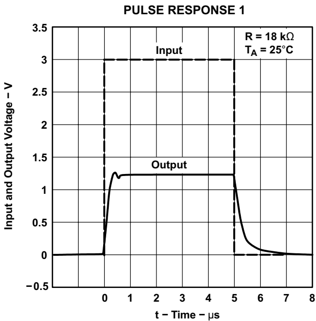
図 5-16. Pulse Response 1
