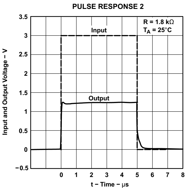
図 5-17. Pulse Response 2
