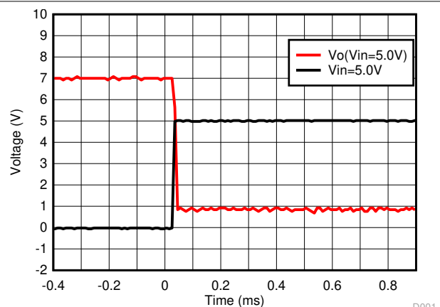
8-4. Output Response with Large Overdrive Voltage
