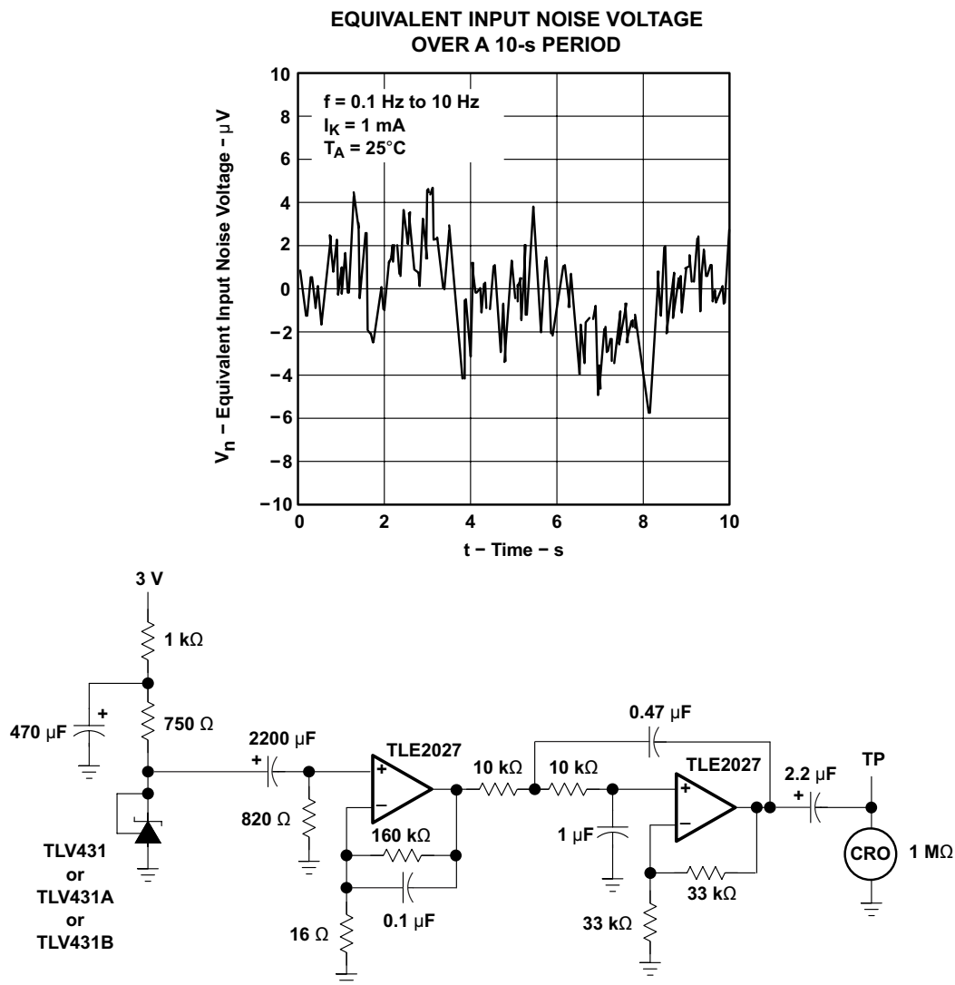
図 5-13. Equivalent Noise Voltage over a 10s Period
