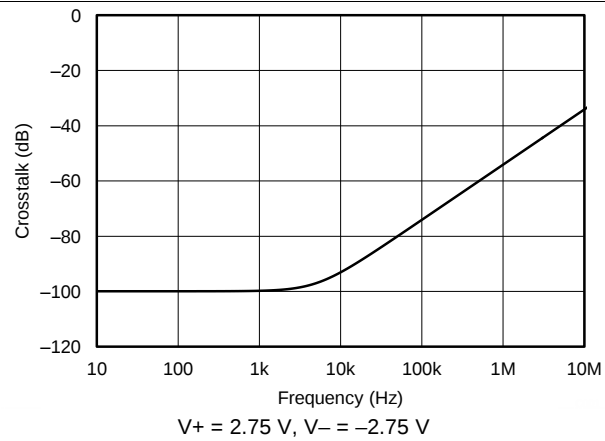
FIG 13. Channel Separation vs Frequency
