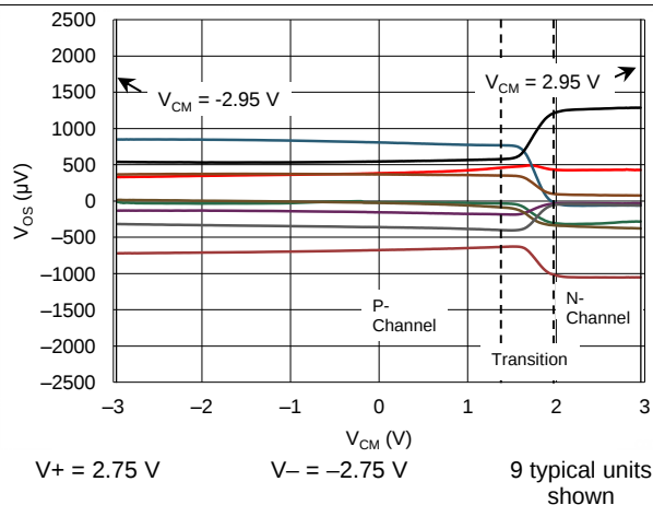
FIG 2. Offset Voltage vs Common-Mode Voltage
