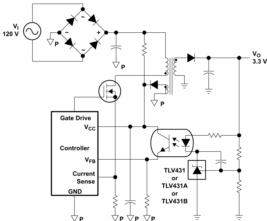
✎ 8-1. Flyback with Isolation Using TLV431, TLV431A, or TLV431B as Voltage Reference and Error Amplifier
