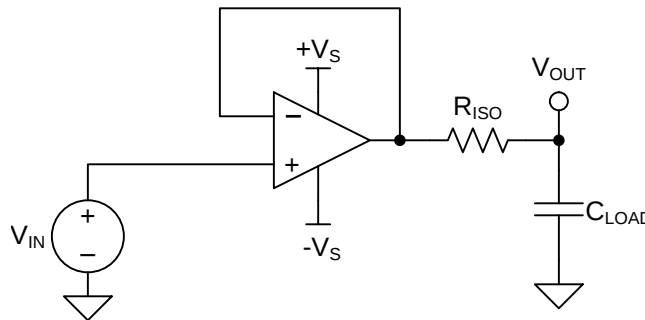
图 30. Unity-Gain Buffer With R_{ISO} Stability Compensation
