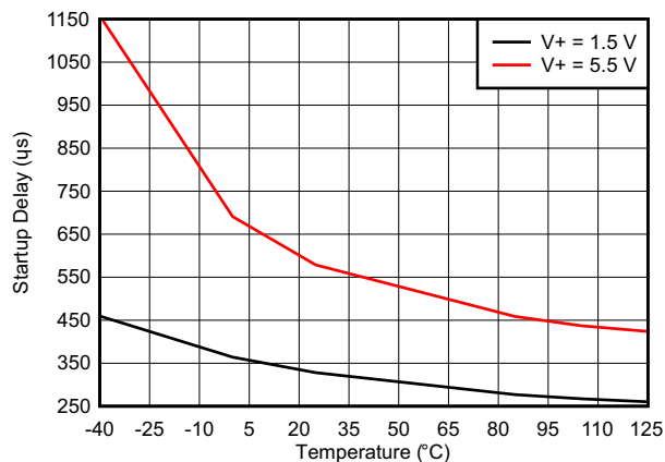
Figure 6-15. Startup Delay
