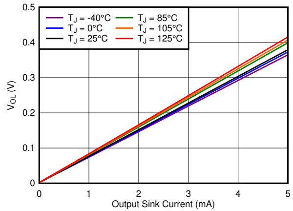
FIG 6-9. Output Voltage Low vs Output Current ( V_+ = 5.5\text{ V} )
