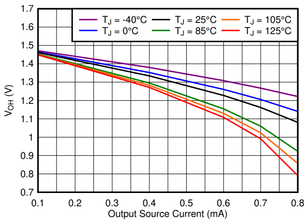
FIG 6-10. Output Voltage High vs Output Current ( V_+ = 1.5\text{ V} )
