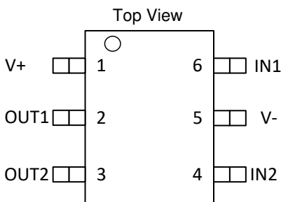
✎ 5-1. DBV Package, 6-Pin SOT-23
