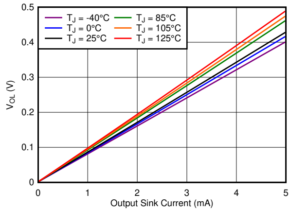
FIG 6-8. Output Voltage Low vs Output Current ( V_+ = 3.3\text{ V} )
