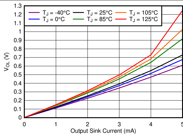
Figure 6-7. Output Voltage Low vs Output Current ( V_+ = 1.5\text{ V} )
