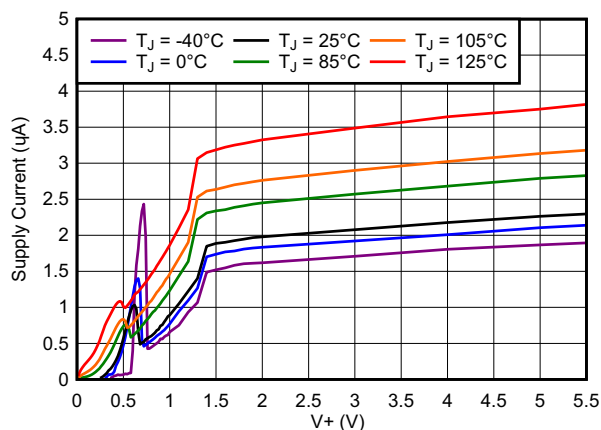
Figure 6-2. Supply Current vs Supply Voltage
