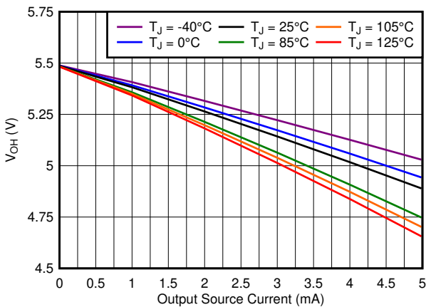
FIG 6-12. Output Voltage High vs Output Current ( V_+ = 5.5\text{ V} )
