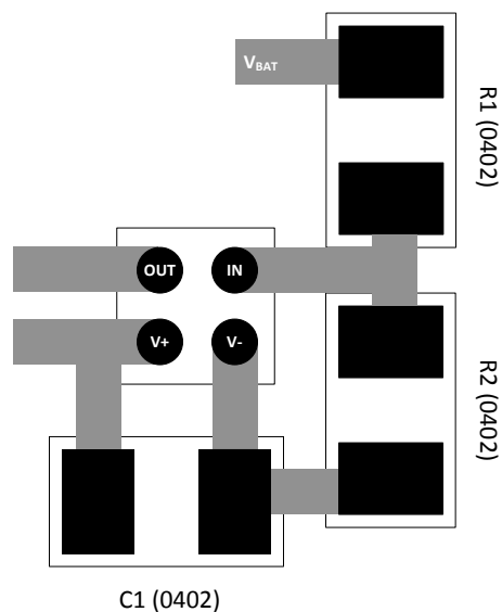
11-1. Layout Example
