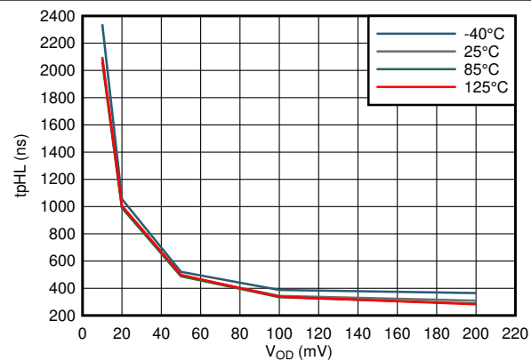
7-29. Propagation Delay High-Low vs Input Overdrive
