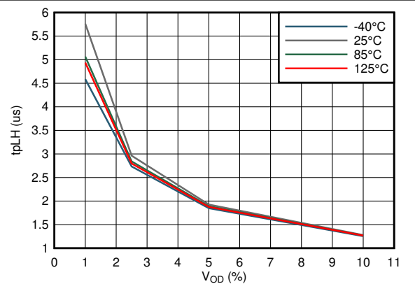
7-28. Propagation Delay Low-High vs Input Overdrive
