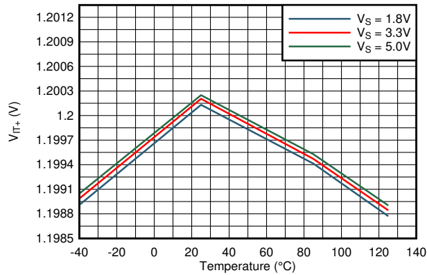
7-1. Positive Threshold vs Temperature
