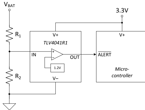
Figure 9-4. Under-Voltage Detection
