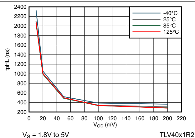
Figure 7-29. Propagation Delay High-Low vs Input Overdrive
