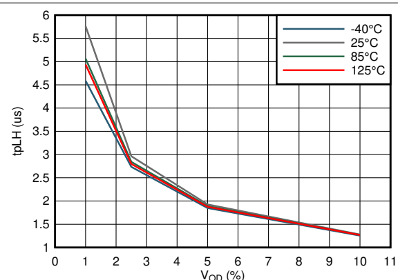
Figure 7-30. Propagation Delay Low-High vs Input Overdrive
