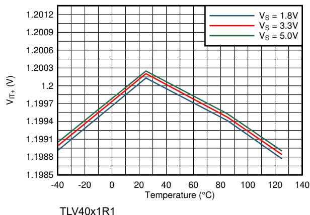
Figure 7-1. Positive Threshold vs Temperature
