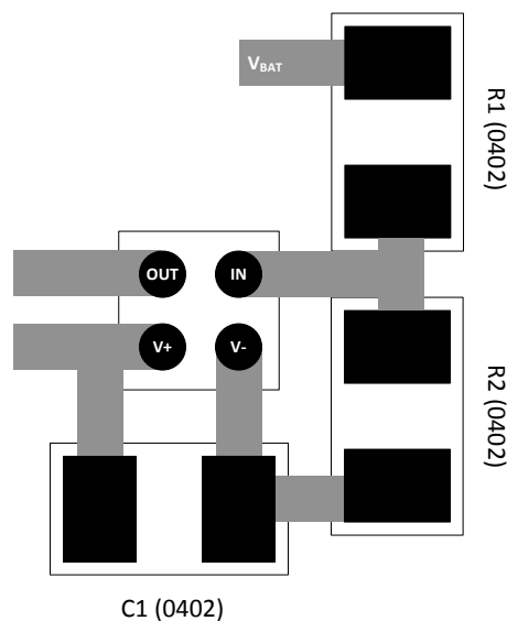
11-1. Layout Example
