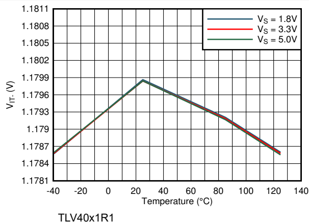
Figure 7-3. Negative Threshold vs Temperature
