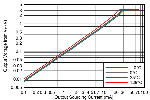
7-22. Output Voltage vs Output Sourcing Current
