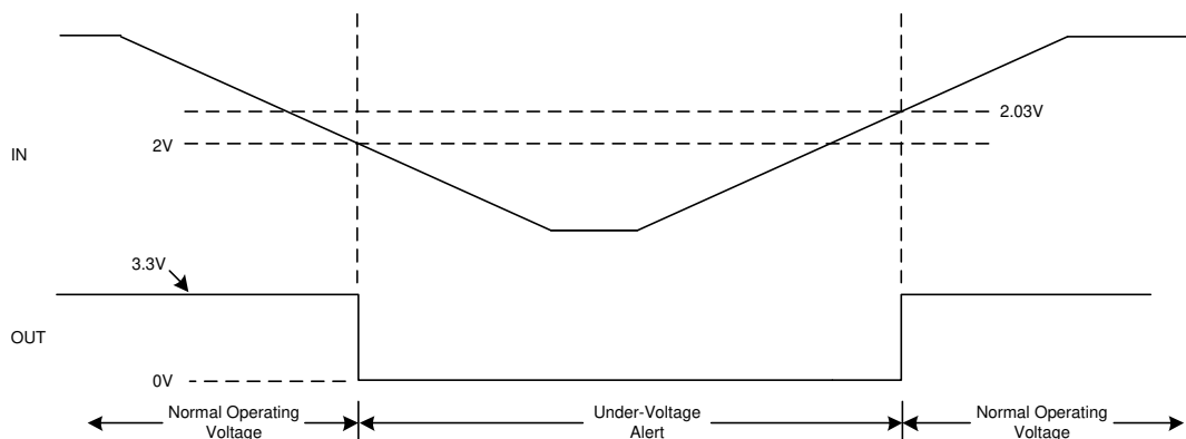
図 9-5. Under-Voltage Detection
