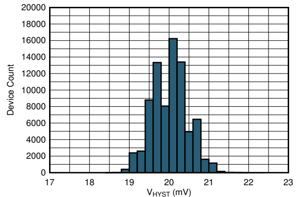
FIG 8-7. V_{HYST} Histogram (TLV40x1R1, V_S=5V )
