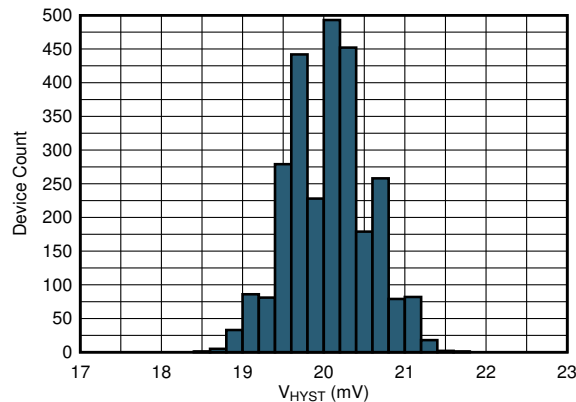
FIG 8-6. V_{HYST} Histogram (TLV40x1R2, V_S=5V )
