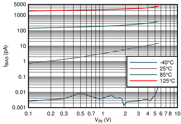
7-19. Bias Current vs Common Mode Voltage
