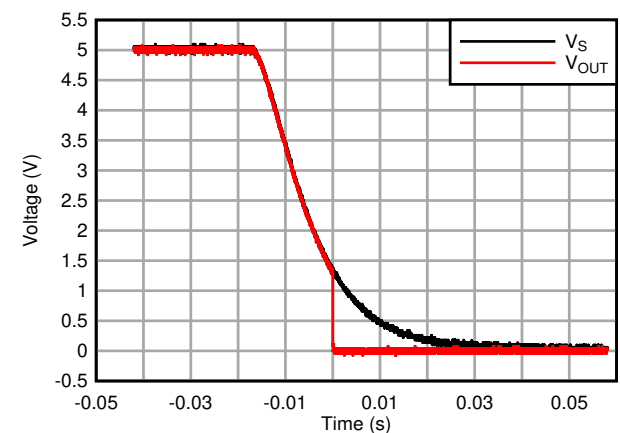
8-4. TLV4041/4051 Output for V_S Falling
