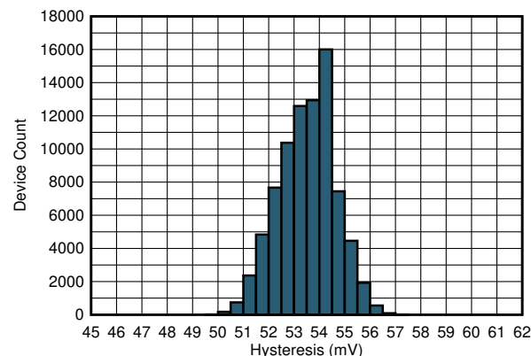
FIG 8-8. V_{HYST} Histogram (TLV40x1S5, V_S=5V )
