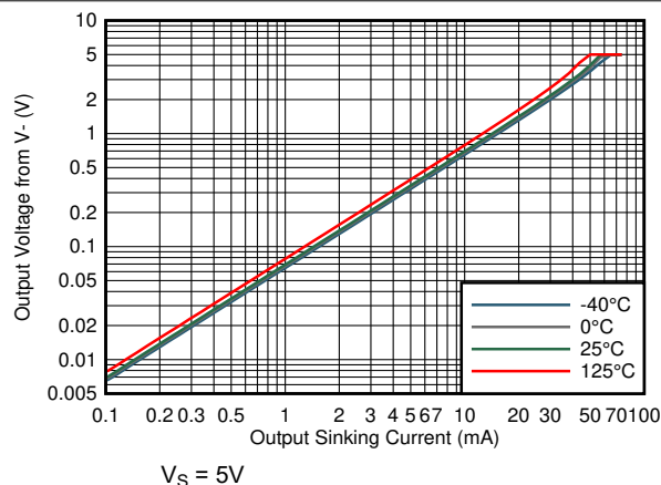
Figure 7-25. Output Voltage vs Output Sinking Current
