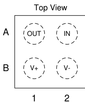
图 5-1. YKA Package 4-Bump DSBGA Top View
