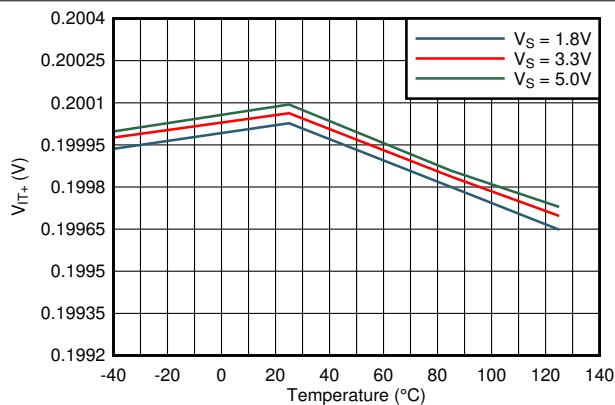
7-7. Positive Threshold vs Temperature
