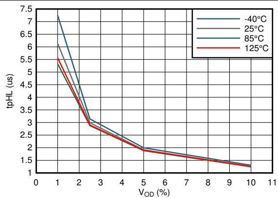
7-31. Propagation Delay High-Low vs Input Overdrive
