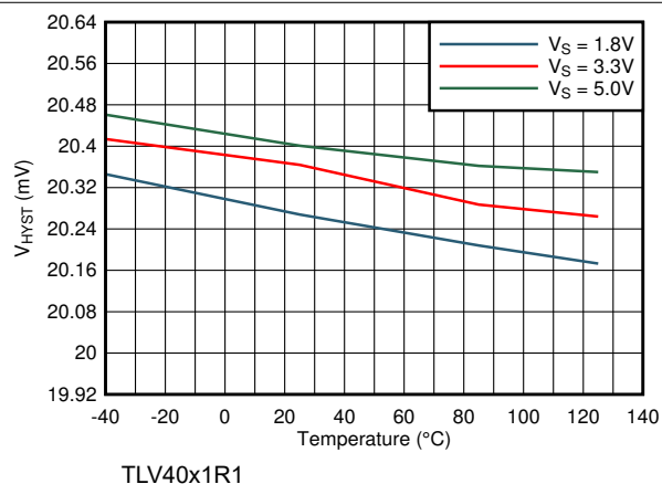
Figure 7-5. Hysteresis vs Temperature
