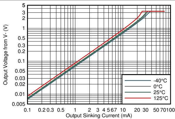
7-21. Output Voltage vs Output Sinking Current
