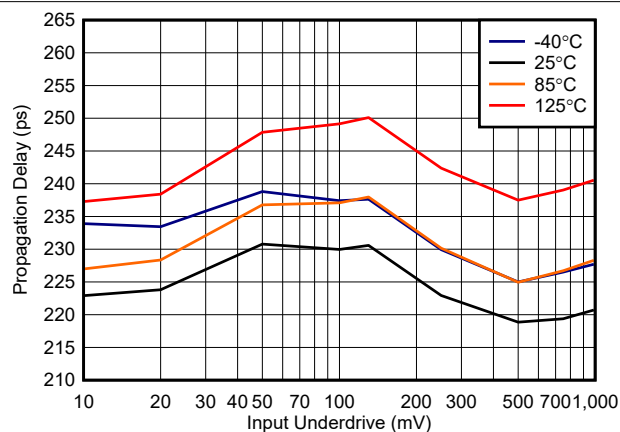
Figure 6-18. Propagation Delay vs. Underdrive, 5 V
