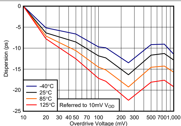
Figure 6-20. Dispersion vs. Overdrive, 5 V
