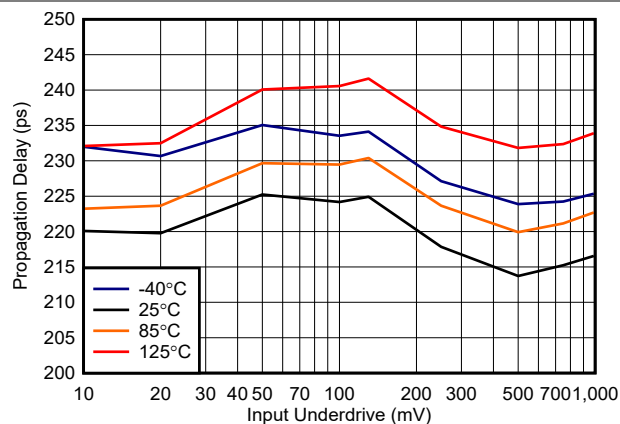
Figure 6-16. Propagation Delay vs. Underdrive, 3.3 V
