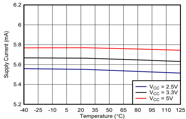
FIG 6-38. TLV3603 Supply Current vs. Temp (Output High)
