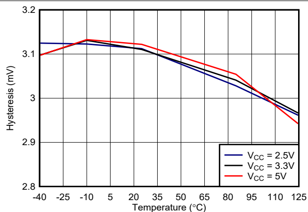
FIG 6-4. TLV3601 Hysteresis vs. Temperature
