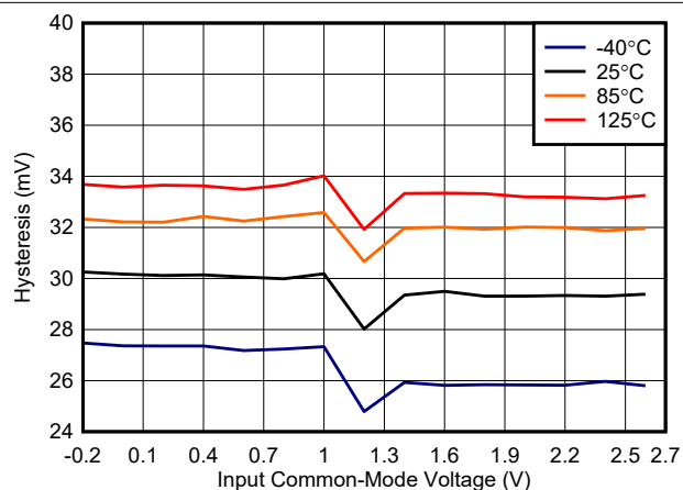
FIG 6-14. TLV3603 Hysteresis vs. Common-Mode, 2.5 V
