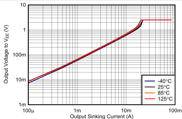
FIG 6-26. Output Voltage vs. Output Sinking Current, 2.5 V
