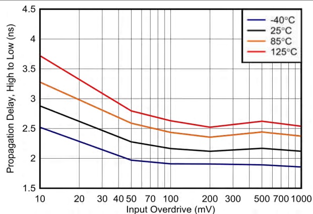
Figure 6-44. Propagation Delay, High to Low, 5 V
