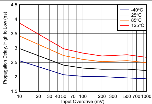
Figure 6-42. Propagation Delay, High to Low, 3.3 V
