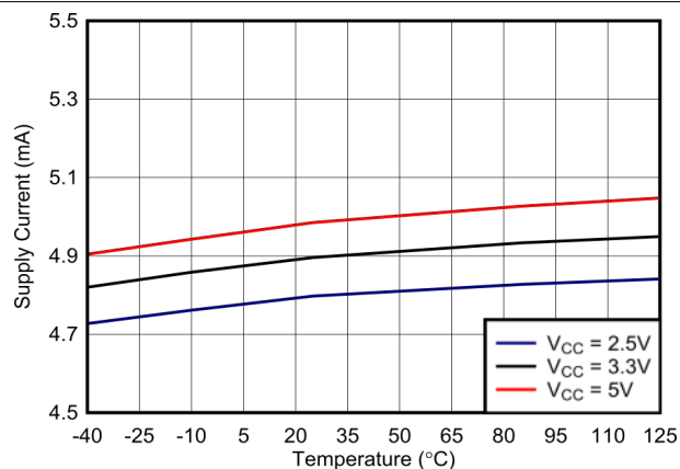
FIG 6-34. TLV3601 Supply Current vs. Temp (Output High)
