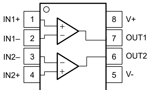
図 5-3. TLV3602 DGK, DSG Packages 8-Pin VSSOP, WSON
