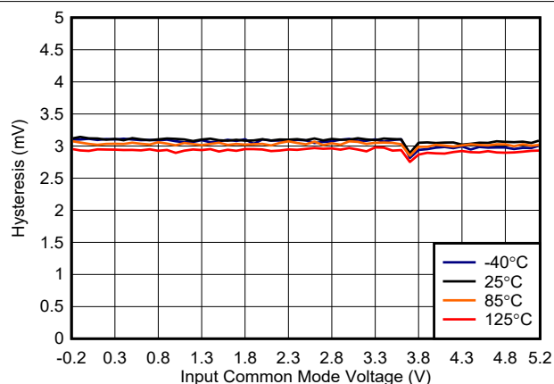
FIG 6-10. TLV3601 Hysteresis vs. Common-Mode, 5 V
