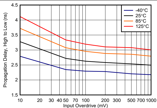
Figure 6-40. Propagation Delay, High to Low, 2.5 V
