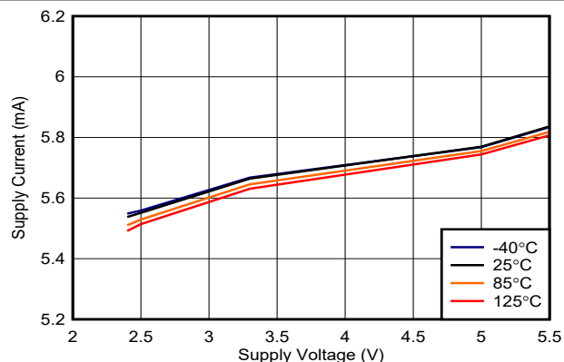
FIG 6-36. TLV3603 Supply Current vs. Voltage (Output High)
