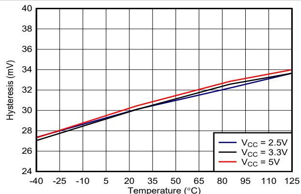
FIG 6-12. TLV3603 Hysteresis vs. Temperature
