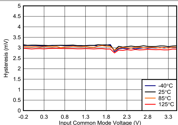
FIG 6-8. TLV3601 Hysteresis vs. Common-Mode, 3.3 V
