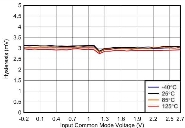
FIG 6-6. TLV3601 Hysteresis vs. Common-Mode, 2.5 V
