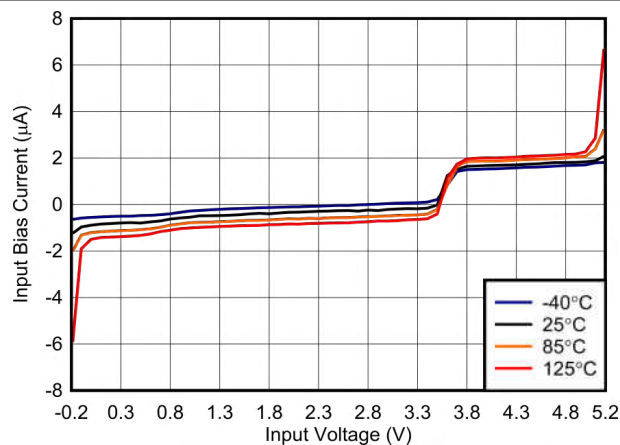
FIG 6-24. Bias Current vs. Input Voltage, 5 V
