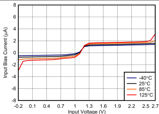
FIG 6-22. Bias Current vs. Input Voltage, 2.5 V
