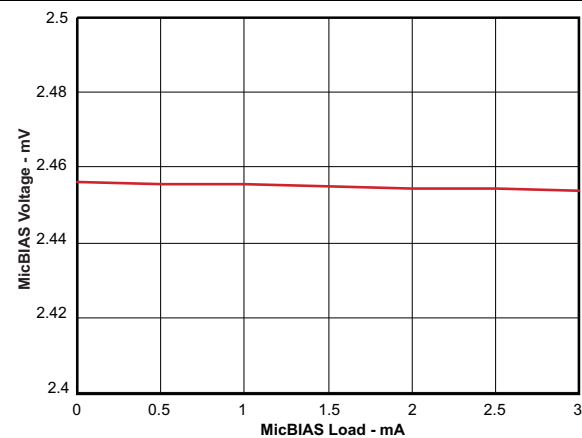
Figure 12. MICBIAS Mode 2, CM = 0.9 V, LDOIN OP Stage vs MICBIAS Load Current
